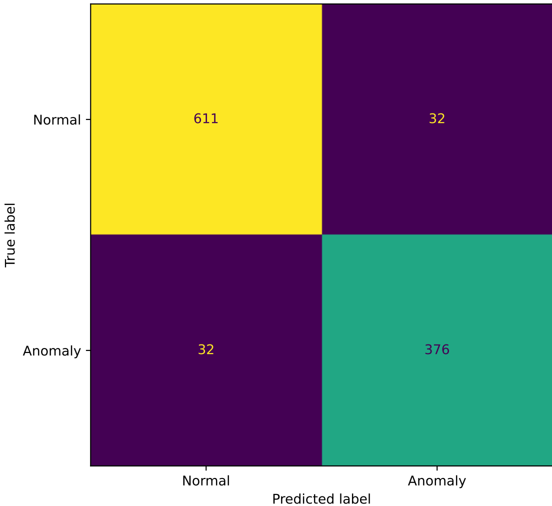
Confusion Matrix - ADMoE-MLP - 12_SpamBase
