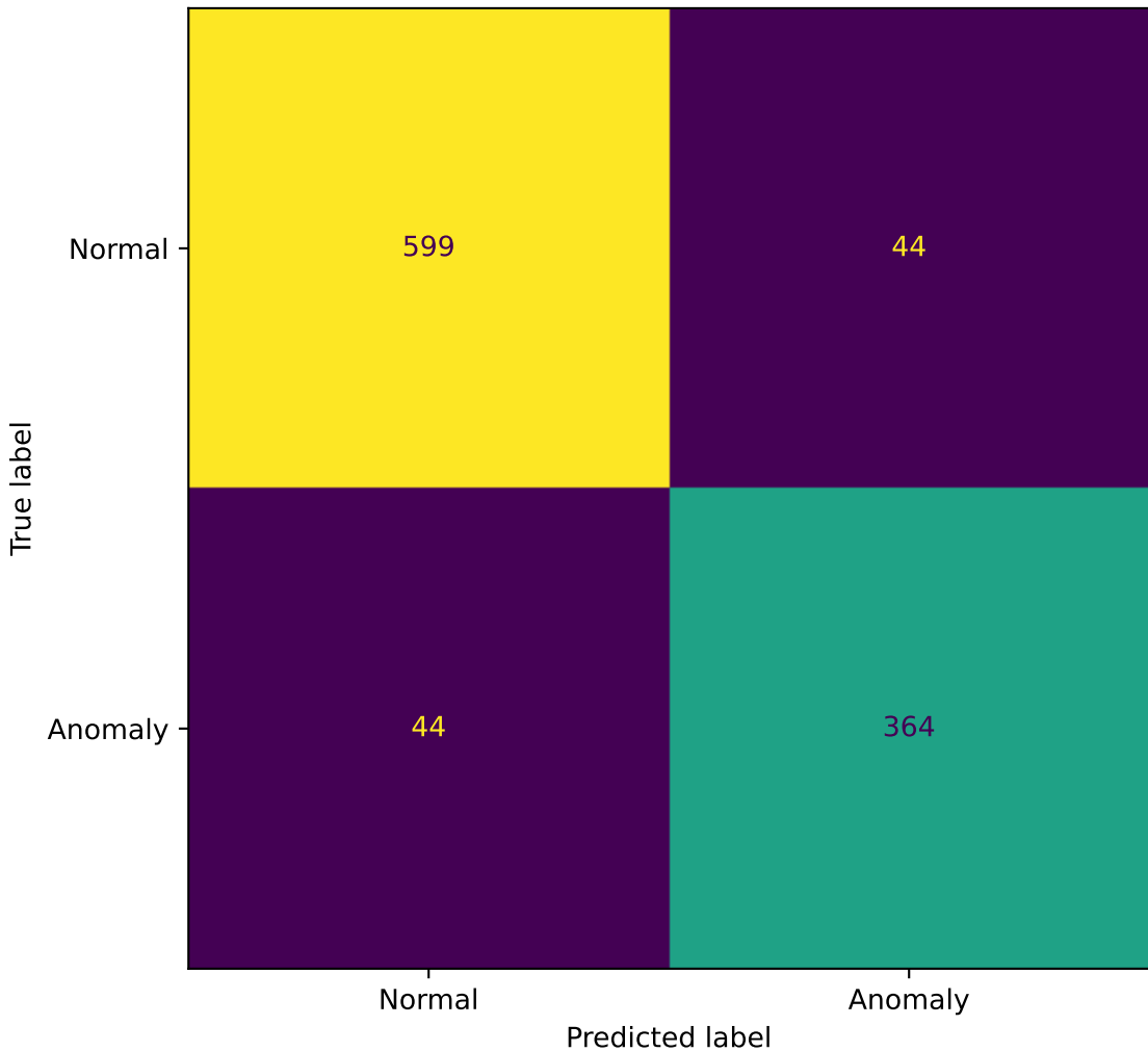
Confusion Matrix - LightGBM - 12_SpamBase
