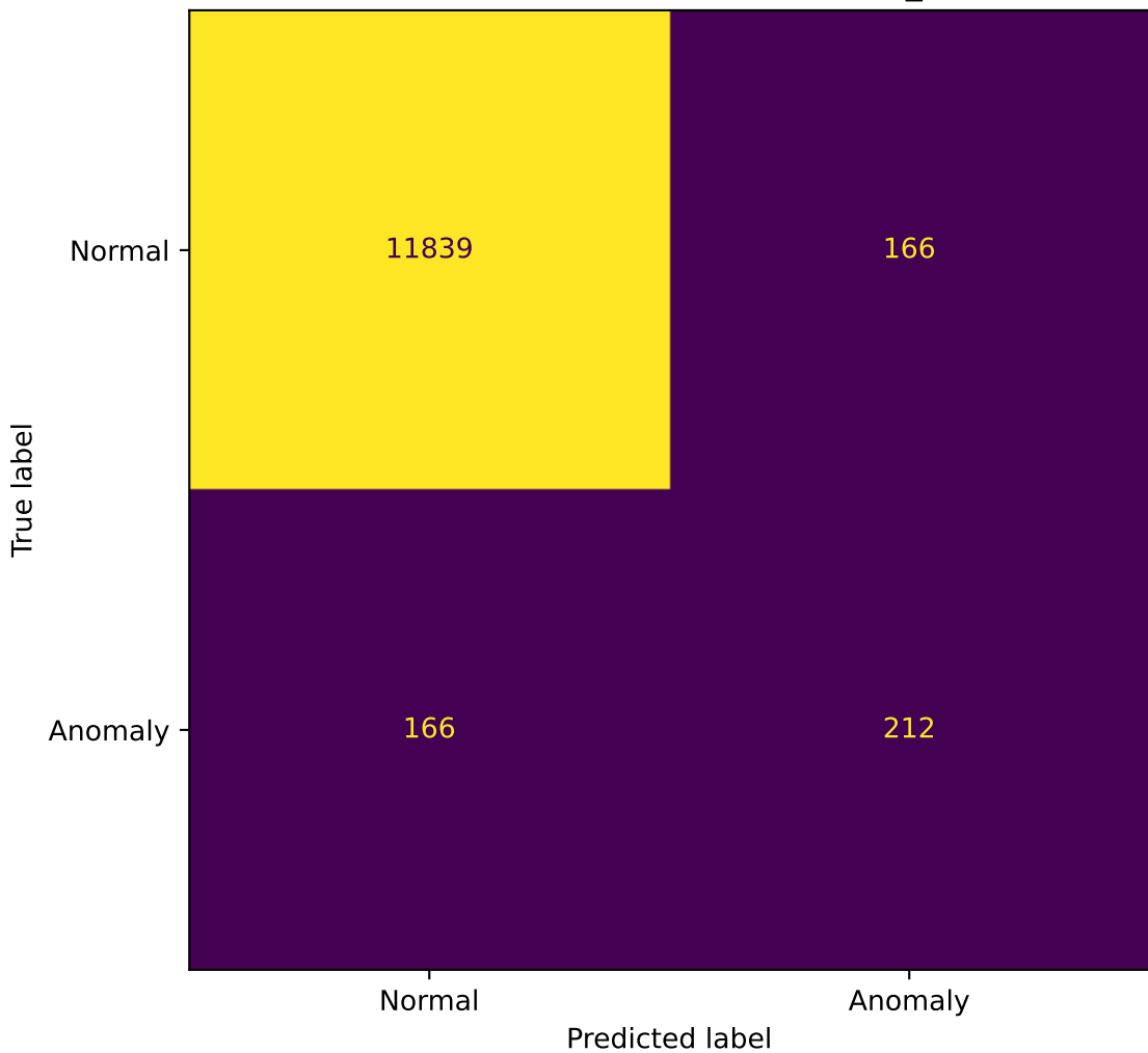
Confusion Matrix - ADMoE-MLP - 1_ALOI
