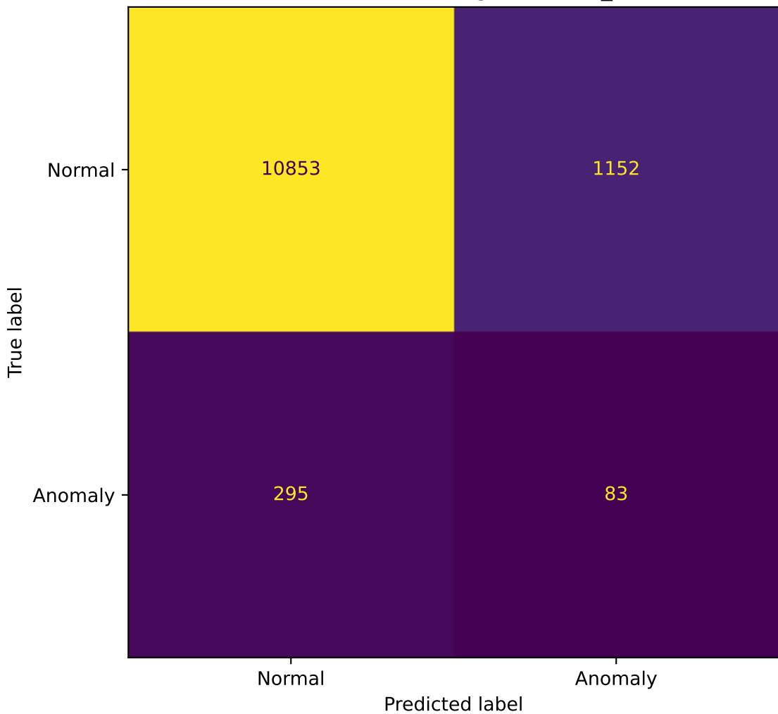
Confusion Matrix - LightGBM - 1_ALOI
