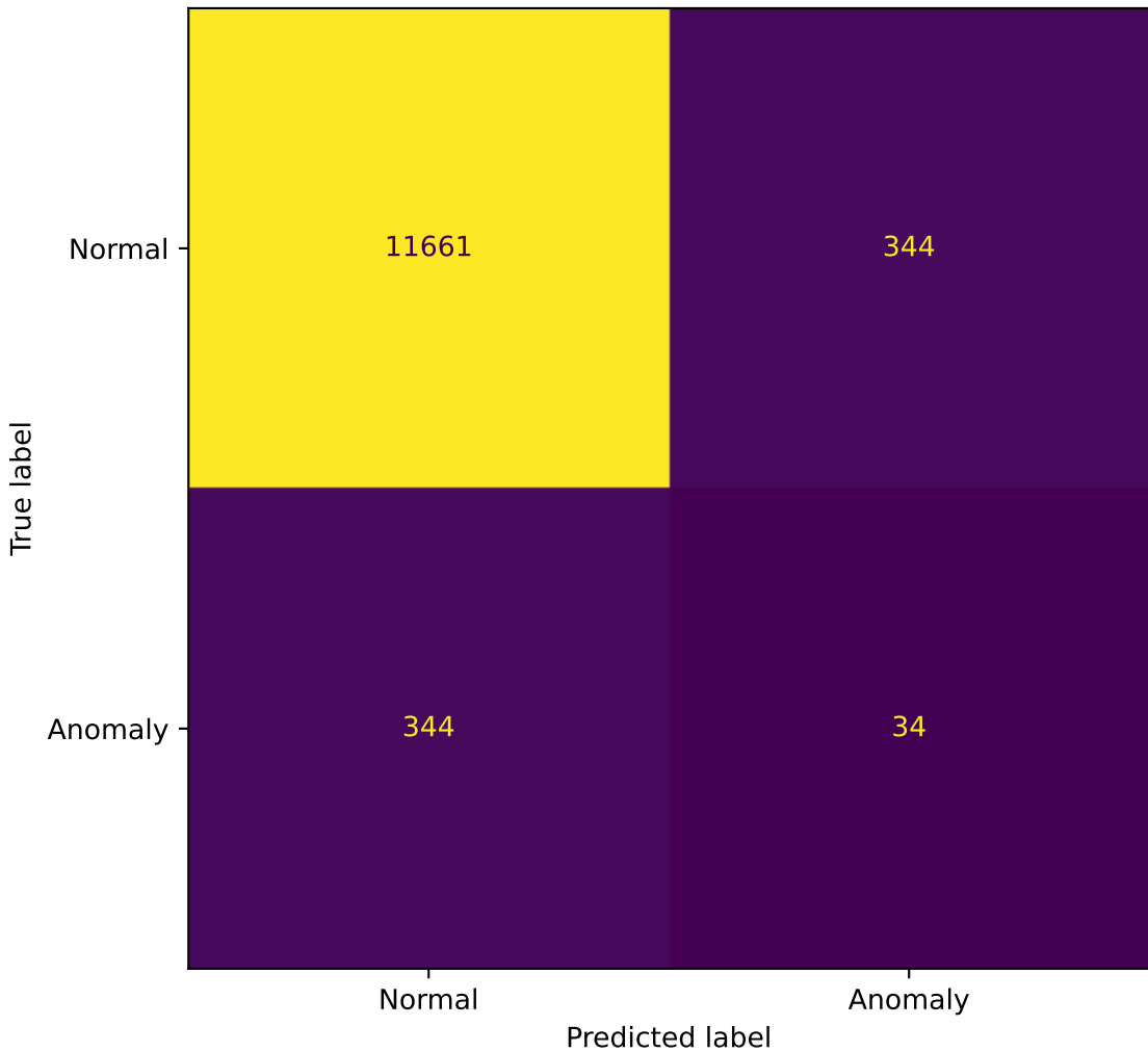
Confusion Matrix - PReNet - 1_ALOI
