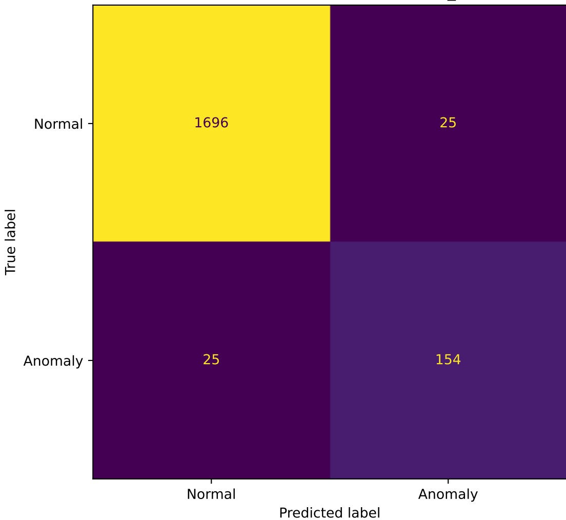
Confusion Matrix - ADMoE-MLP - 27_mnist
