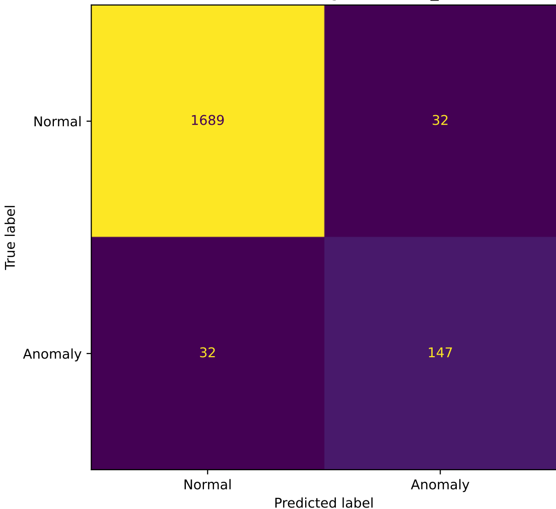
Confusion Matrix - LightGBM - 27_mnist
