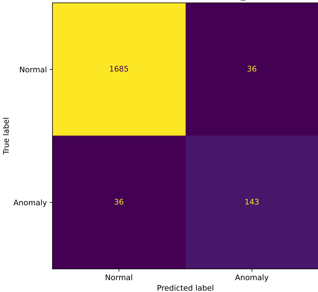
Confusion Matrix - PReNet - 27_mnist
