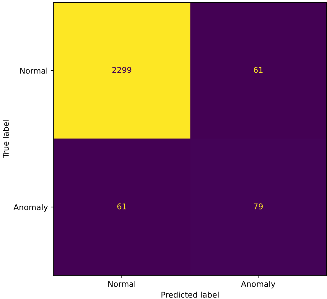
Confusion Matrix - ADMoE-MLP - agnews_0
