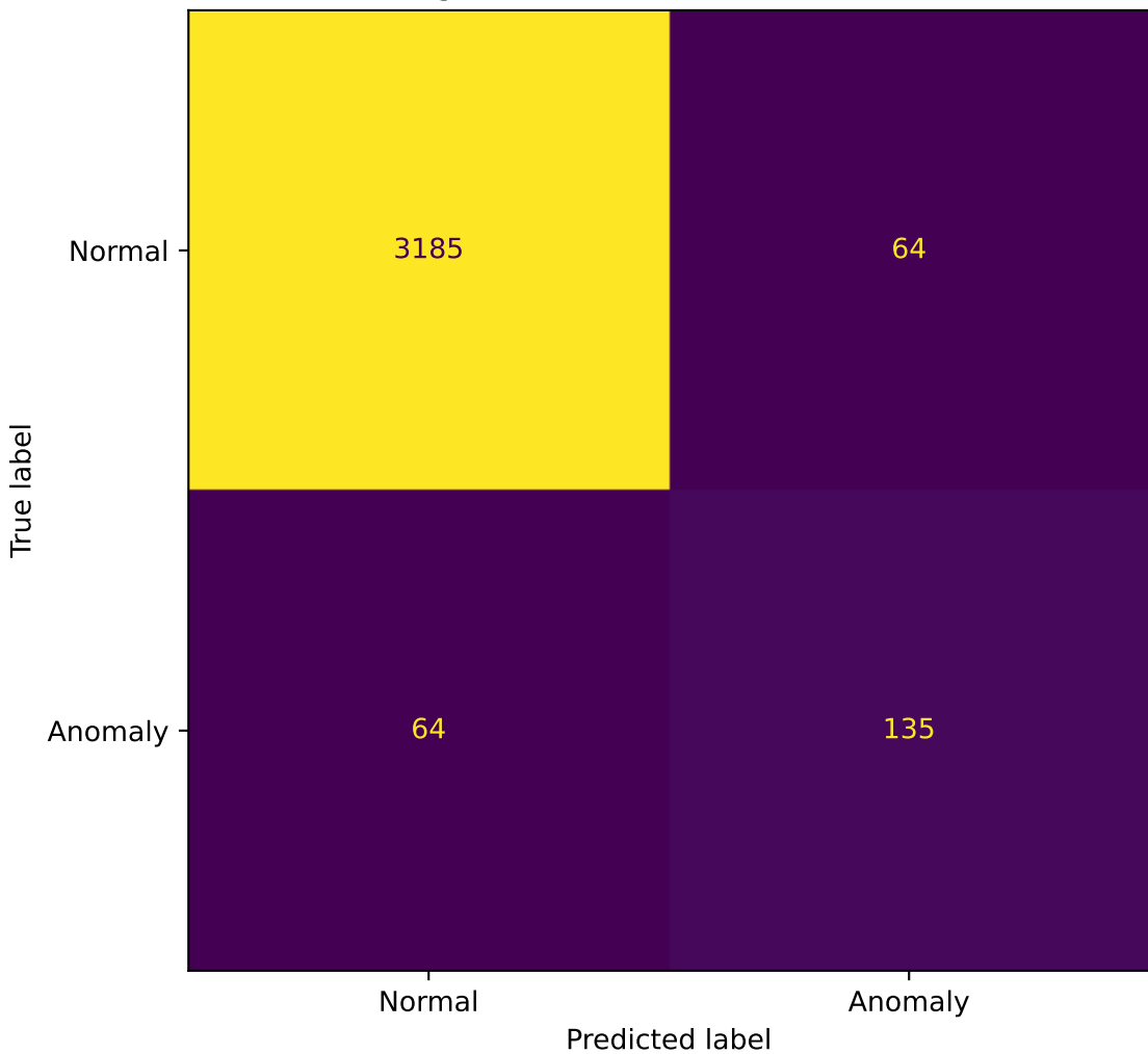
Average Confusion Matrix - ADMoE-MLP
