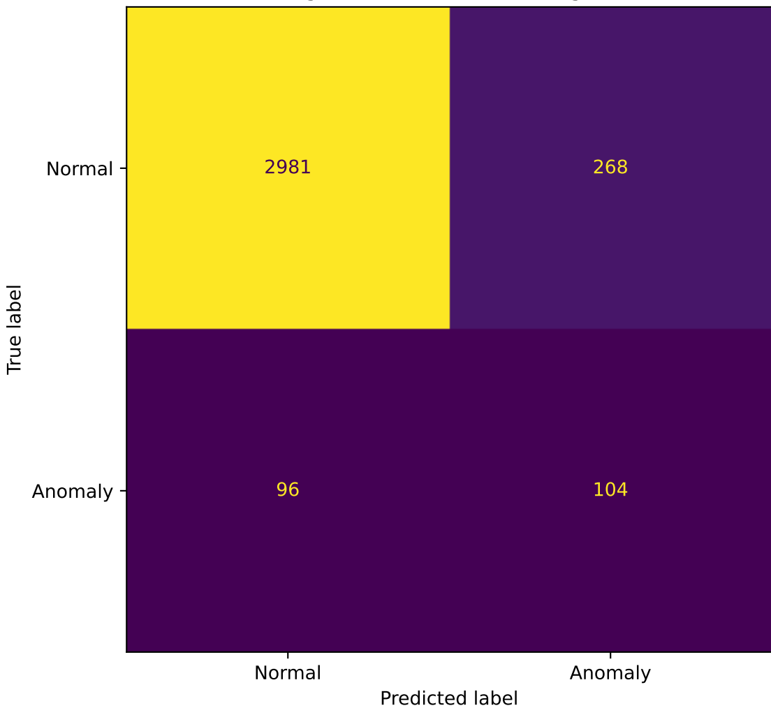
Average Confusion Matrix - LightGBM
