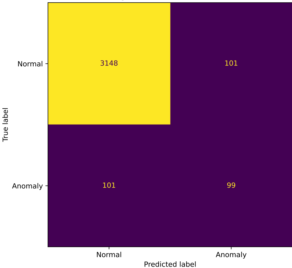
Average Confusion Matrix - PReNet
