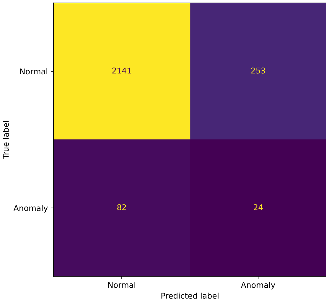
Confusion Matrix - LightGBM - imdb
