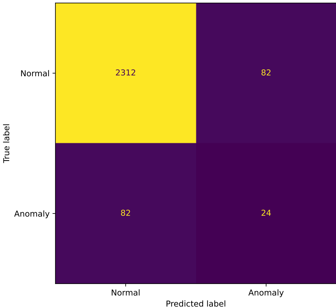
Confusion Matrix - PReNet - imdb
