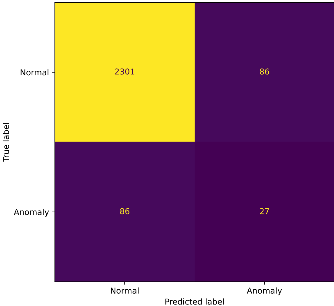
Confusion Matrix - LightGBM - yelp
