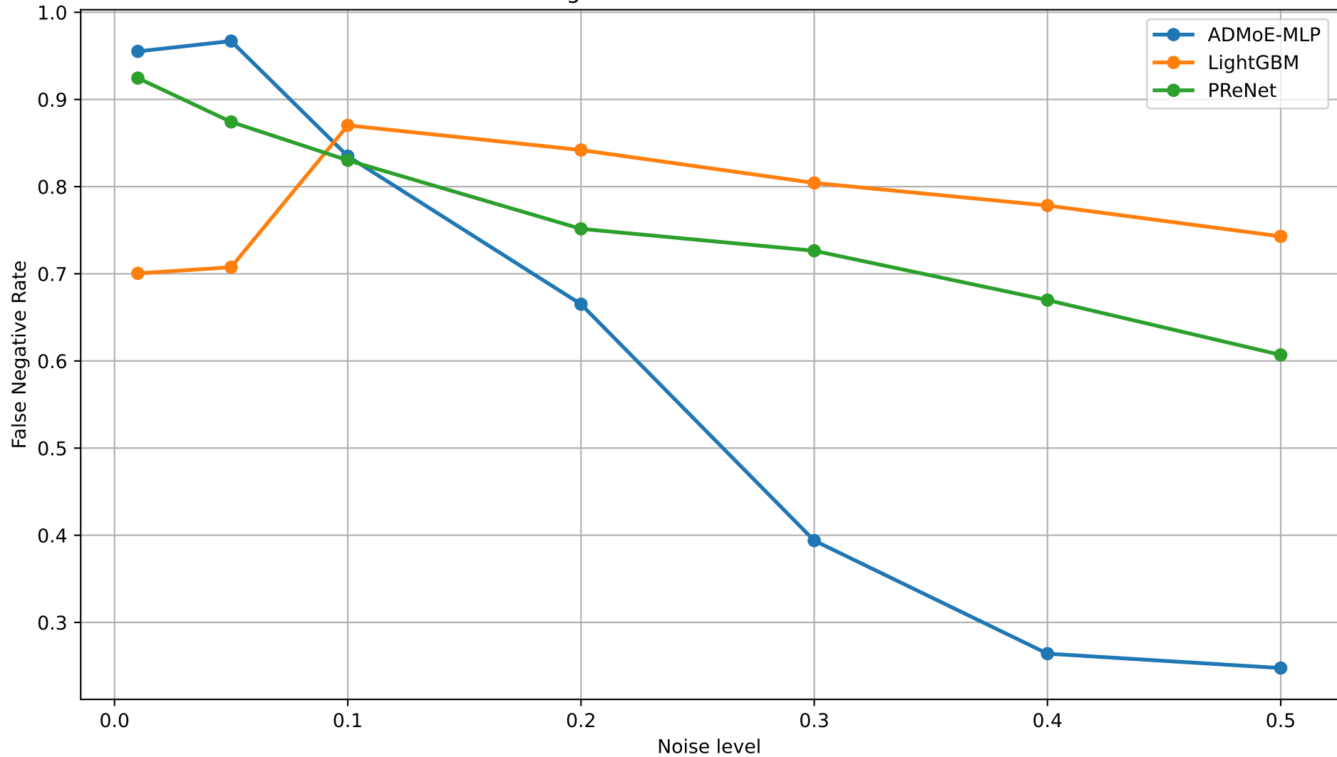
False Negative Rate vs Noise Level - imdb
