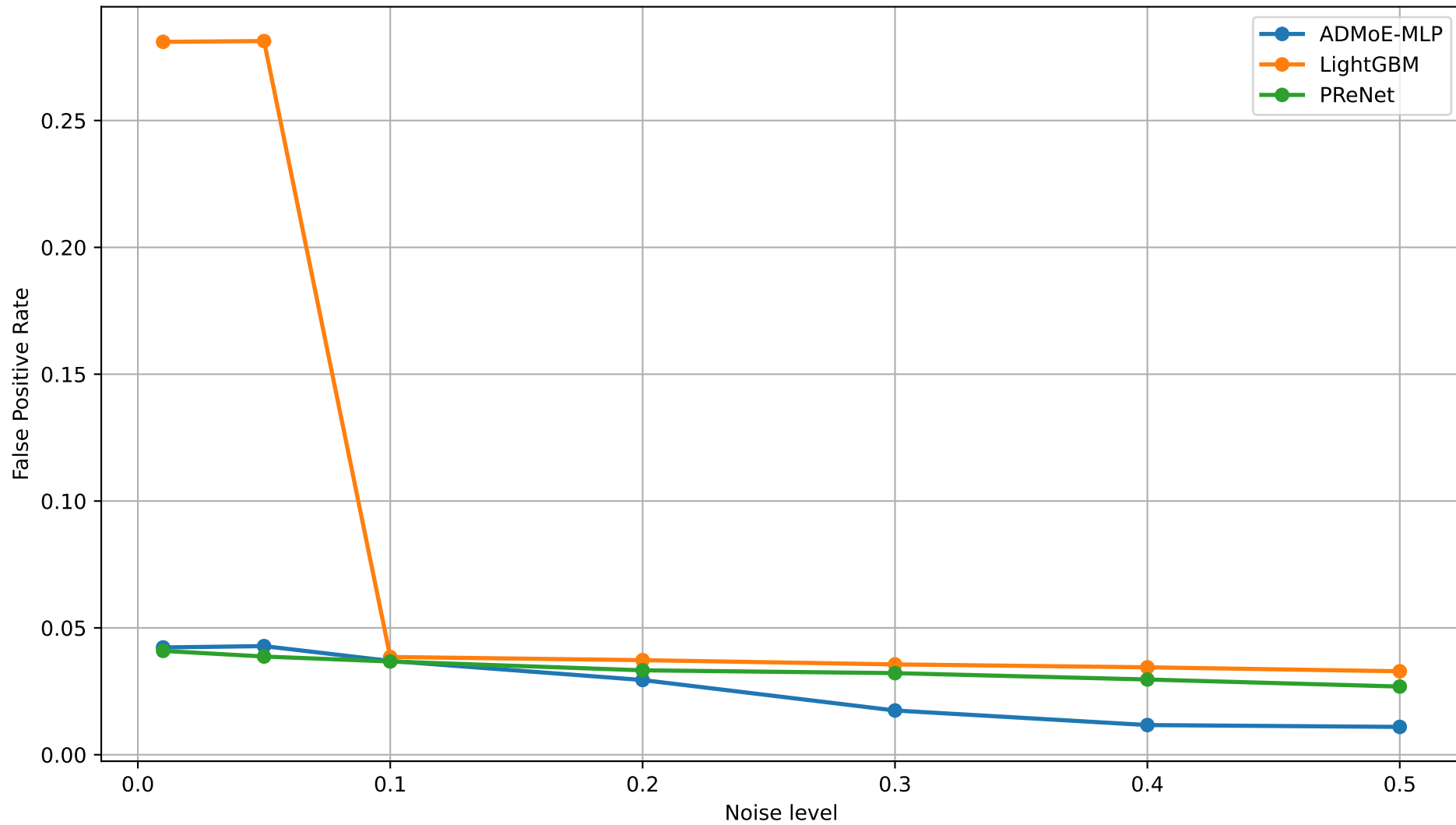
False Positive Rate vs Noise Level - imdb
