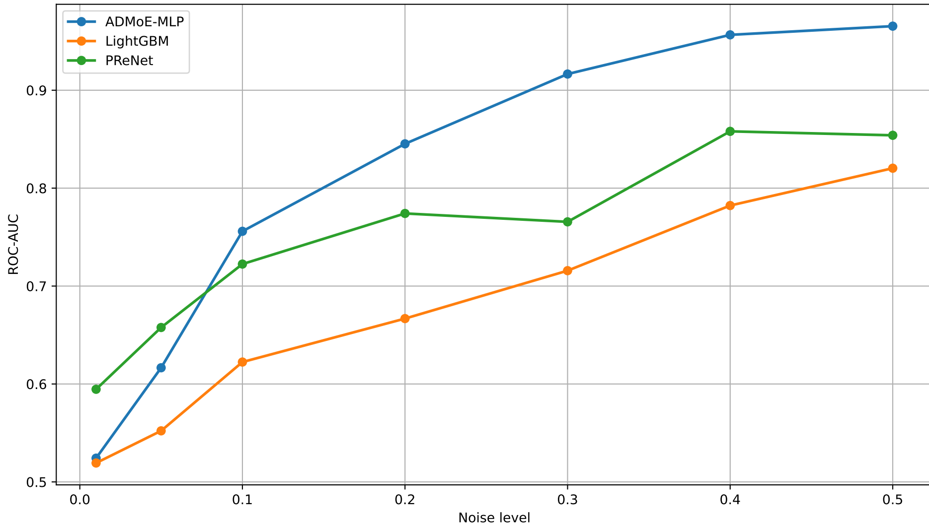
ROC-AUC vs Noise Level - imdb
