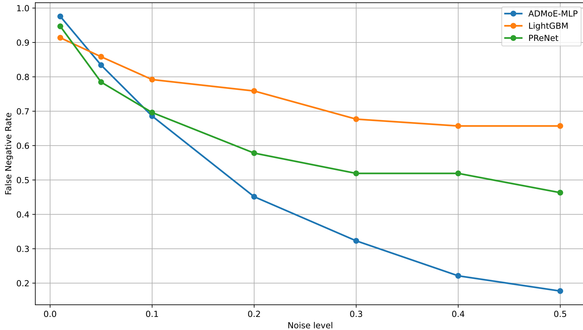
False Negative Rate vs Noise Level - yelp
