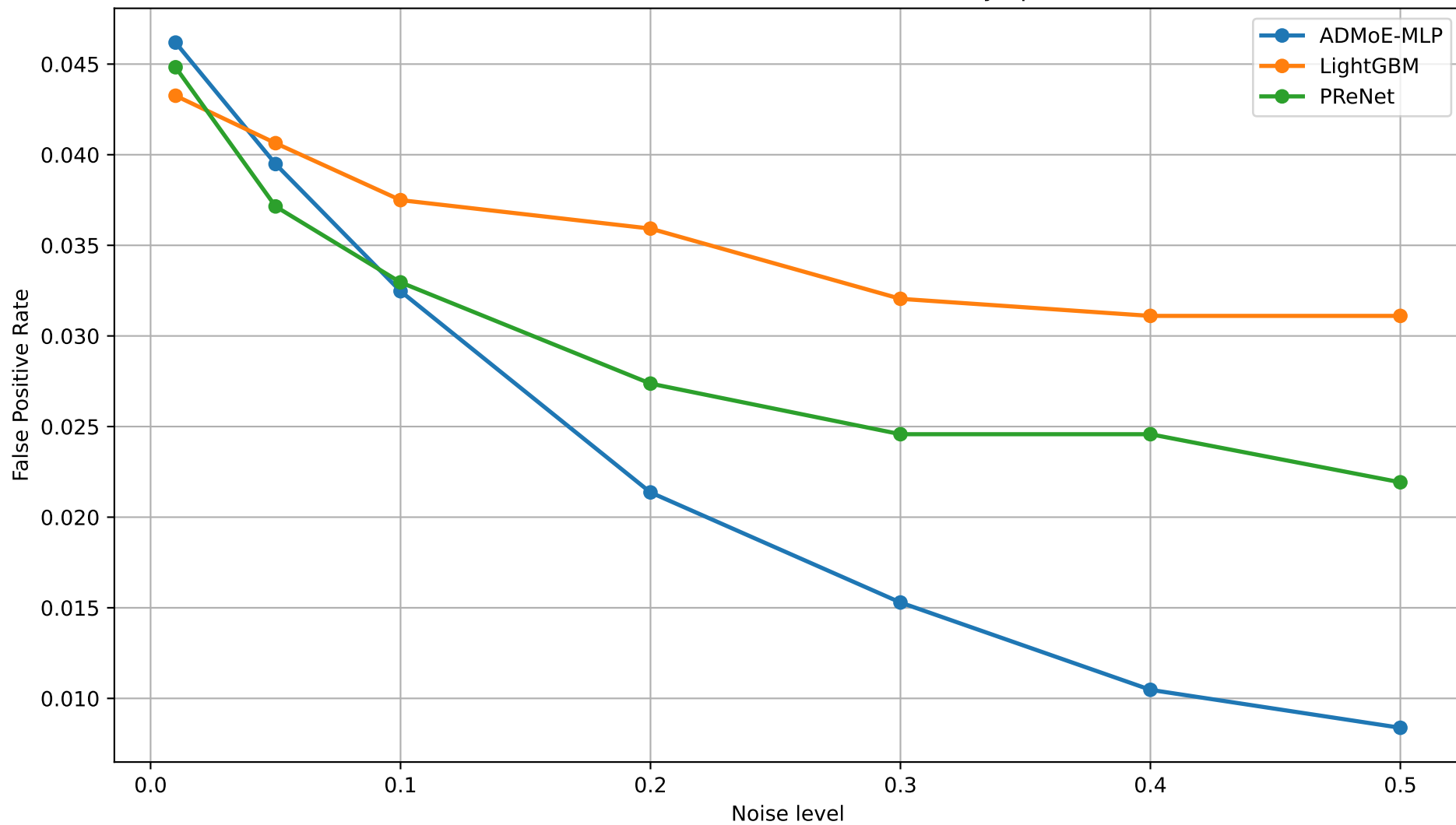
False Positive Rate vs Noise Level - yelp
