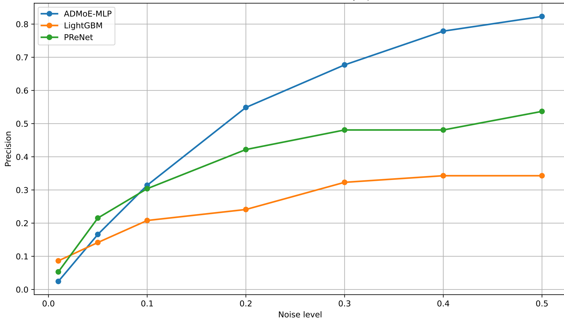
Precision vs Noise Level - yelp
