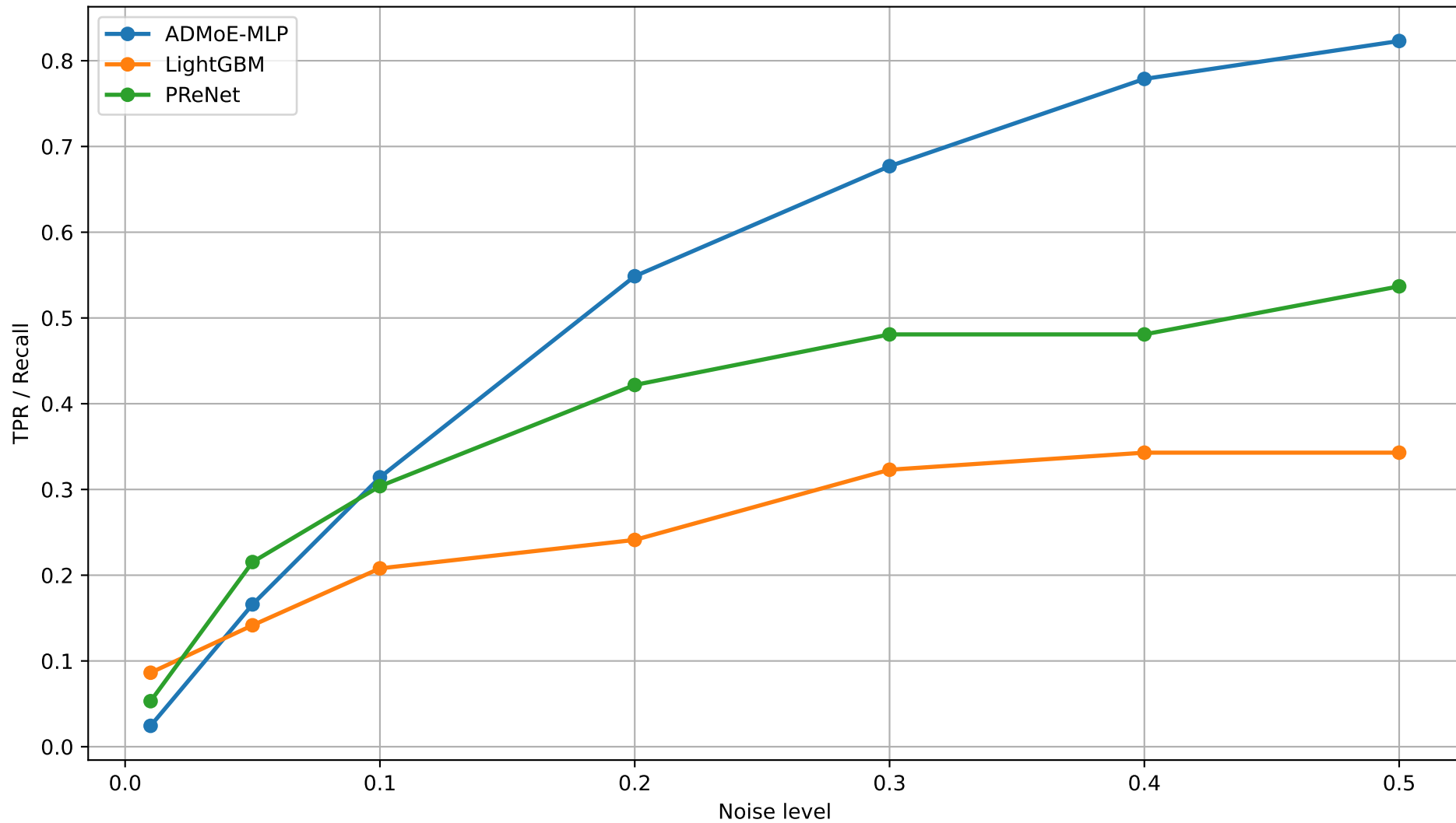
TPR / Recall vs Noise Level - yelp
