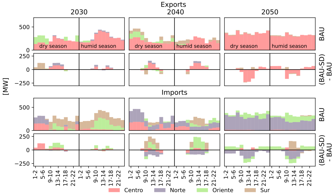
Figure 5: Daily profiles of inter regional exports and imports of power flow for BAU scenario (first and third row), and differences for BAU-SD scenario (second and fourth row)
