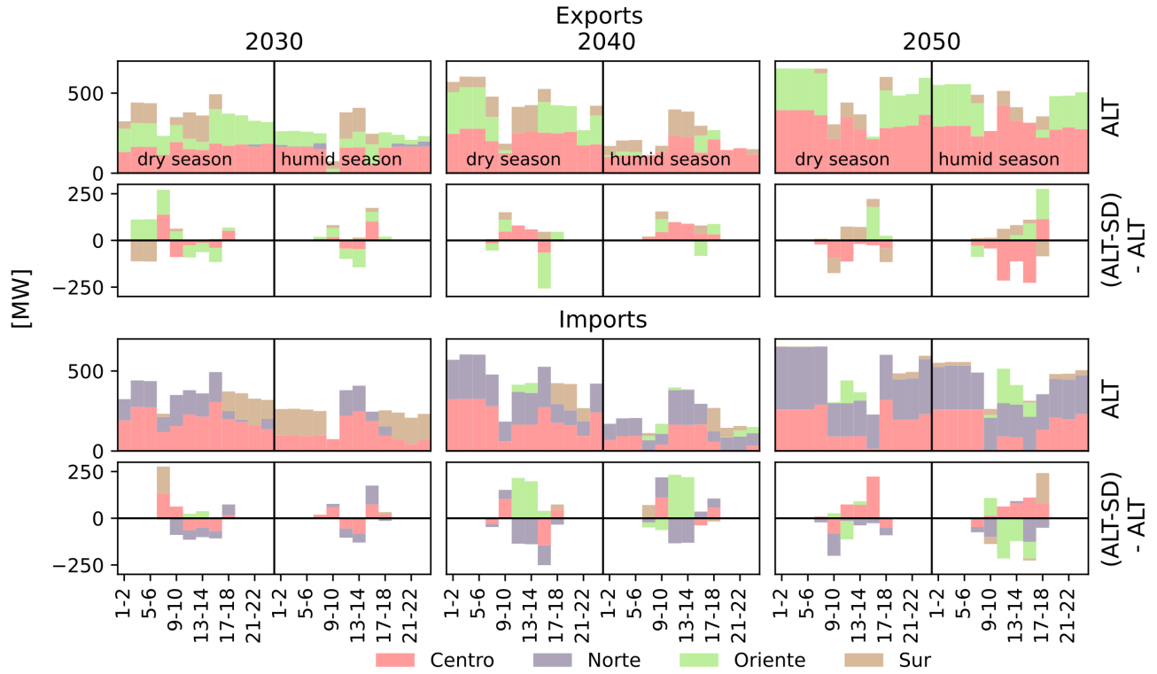
Figure 7: Daily profiles of inter regional exports and imports of power flow por ALT scenario (first and third row), and differences for ALT-SD scenario (second and fourth row)
