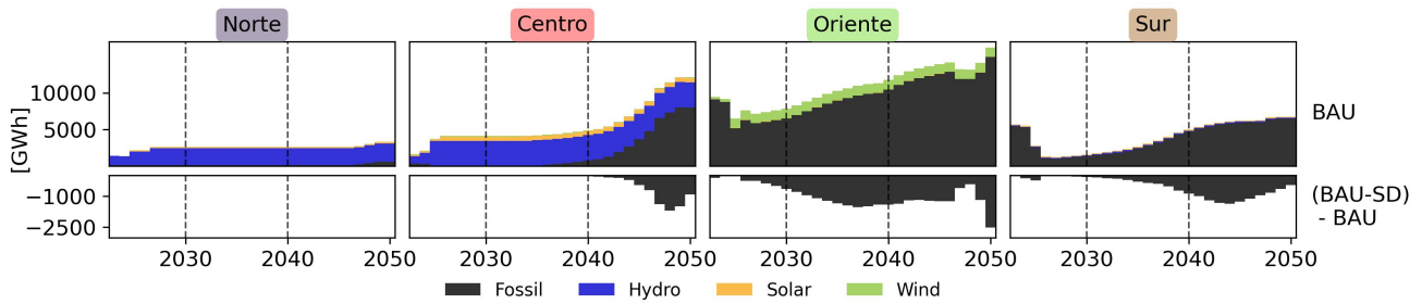
Figure 6: Evolution of regional projected annual electricity generation according to BAU scenario (upper row), and differences for BAU-SD scenario (lower row)
