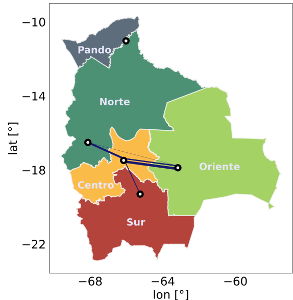
Figure 1: Regional nodes included in the model and power lines
