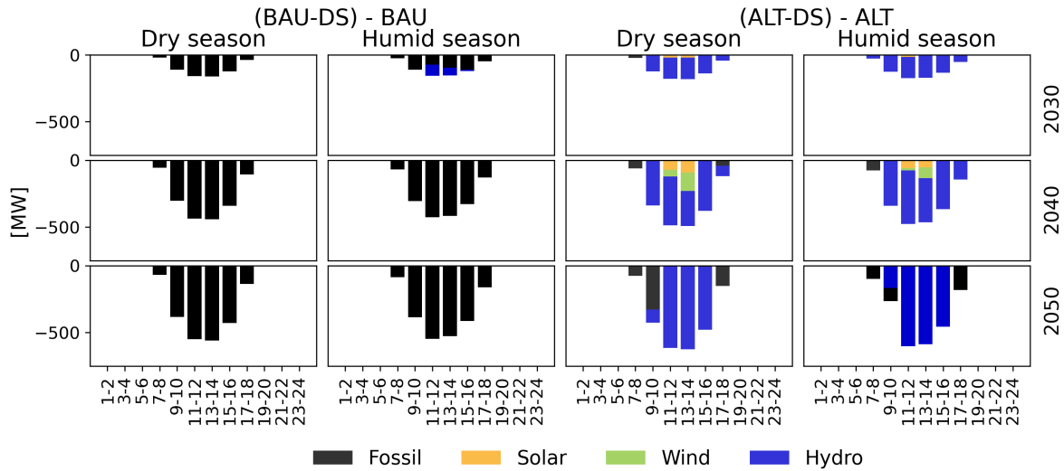
Figure 10: Difference in hourly power output of centralized generation units between BAU-DS/ALT-DS and BAU/ALT scenarios
