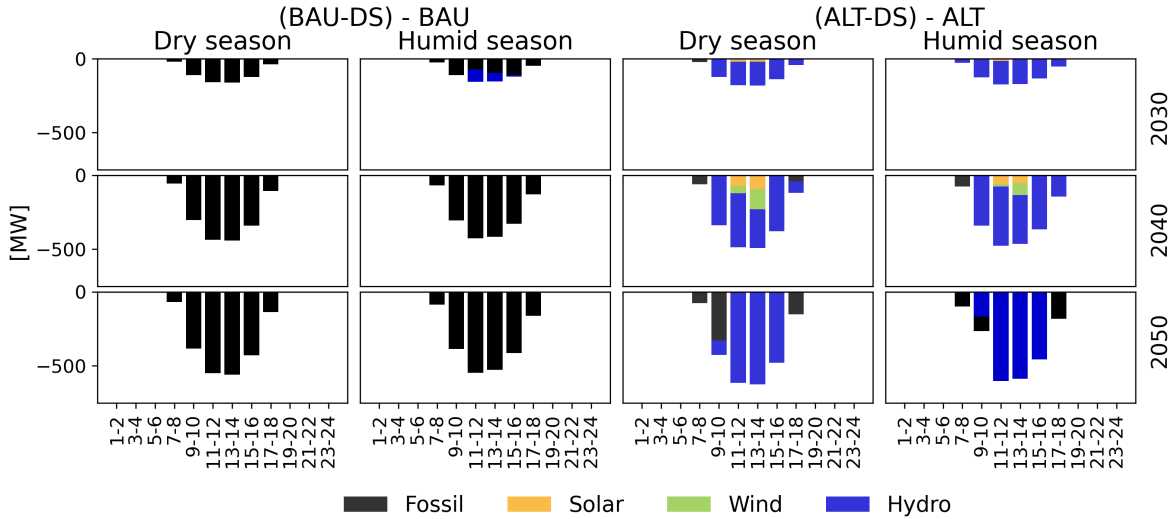
Figure 9: Difference in hourly power output of centralized generation units between BAU-DS/ALT-DS and BAU/ALT scenarios
