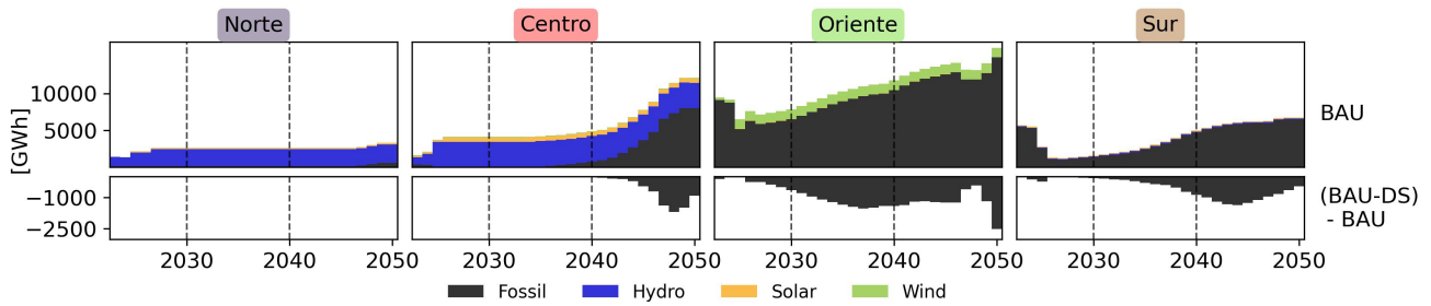
Figure 6: Evolution of regional projected annual electricity generation according to BAU scenario (upper row), and differences for BAU-DS scenario (lower row)
