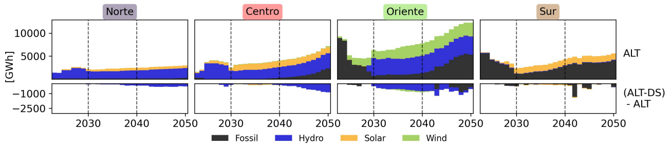
Figure 8: Evolution of regional projected annual electricity generation according to ALT scenario (upper row), and differences for ALT-DS scenario (lower row)
