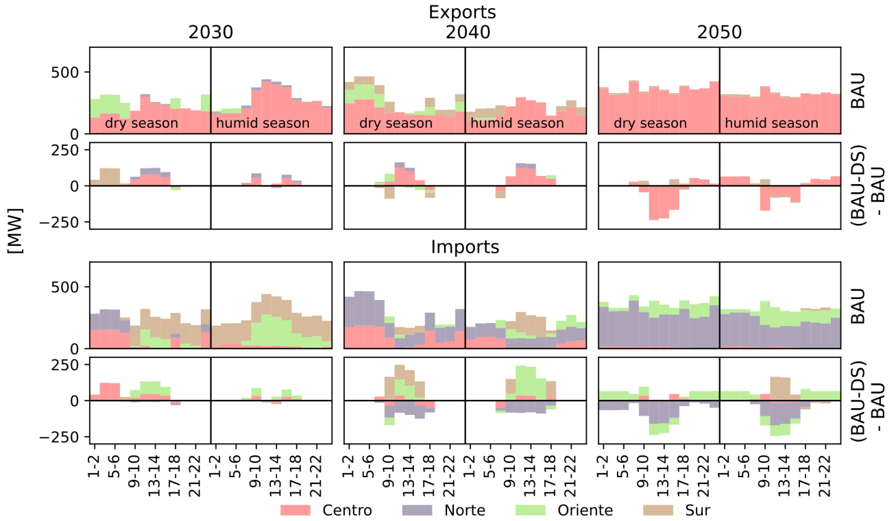
Figure 5: Daily profiles of inter regional exports and imports of power flow for BAU scenario (first and third row), and differences for BAU-DS scenario (second and fourth row)
