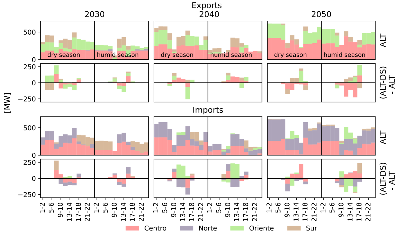
Figure 7: Daily profiles of inter regional exports and imports of power flow por ALT scenario (first and third row), and differences for ALT-DS scenario (second and fourth row)
