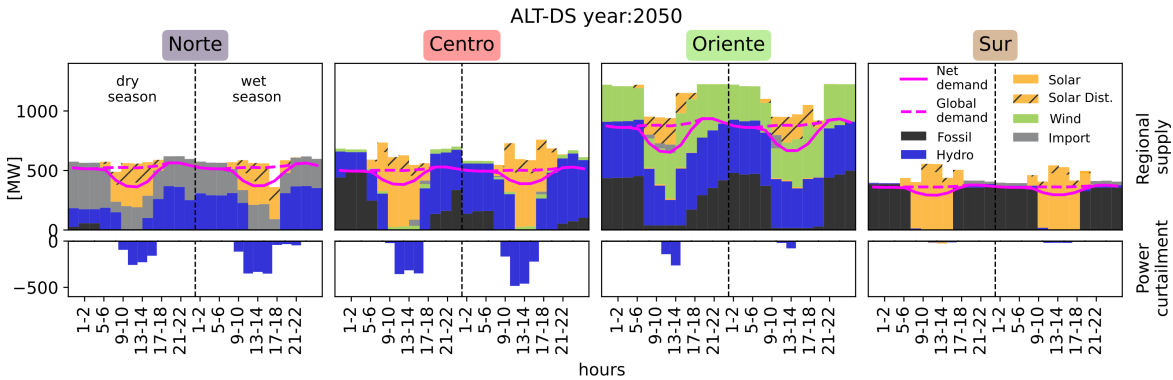
Figure 10: Hourly regional power supply (top row) and curtailed power (bottom row) for ALT-DS scenario and year 2050
