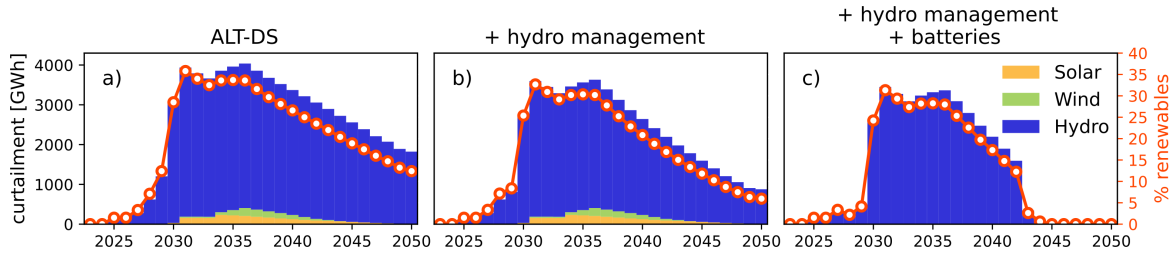
Figure 11: Annual curtailed energy for ALT-DS scenario (a), after the implementation of the alternative hydro operation scheme (b) and the endogenous battery capacity addition (c)
