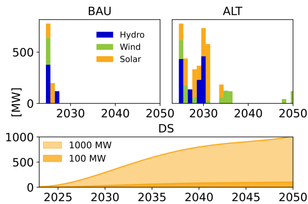
Figure 3: Centralized generation capacity additions for BAU and ALT scenarios (top row), and for DS generation (below)
