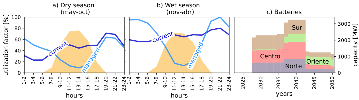
Figure 5: Current (blue line) and proposed (sky blue line) hydro hourly operation schemes and solar utilization factor (yellow area) for dry (a) and wet (b) seasons. Endogenous battery capacity additions (c)
