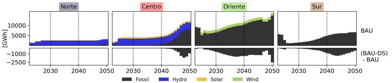
Figure 7: Evolution of regional projected annual electricity generation according to BAU scenario (upper row), and differences for BAU-DS scenario (lower row)
