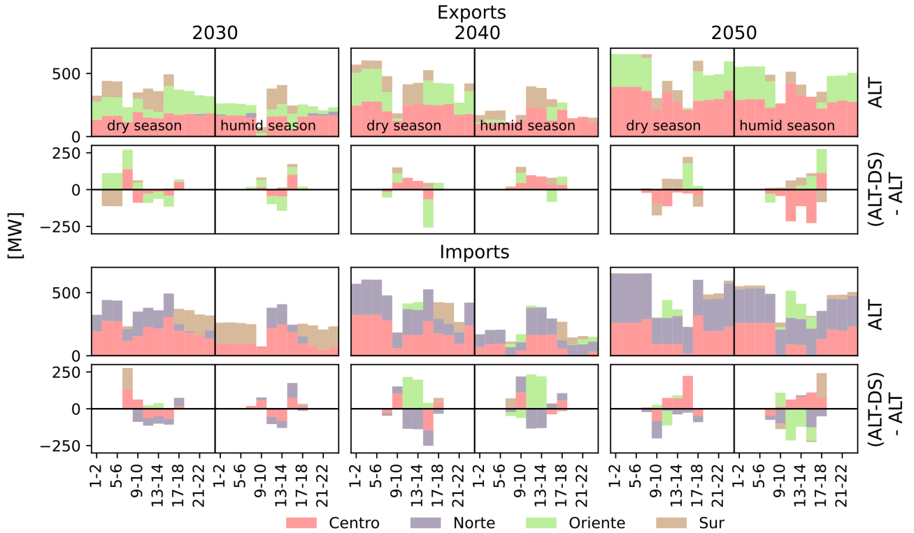
Figure 8: Daily profiles of inter regional exports and imports of power flow for ALT scenario (first and third row), and differences for ALT-DS scenario (second and fourth row)
