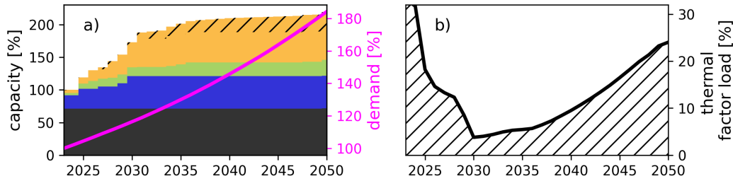
Figure 12: Total installed capacity (shadowed areas) and power demand (magenta line) as percentage of the base year (a) and annual load factor of thermal power plants (b) for ALT-DS scenario
