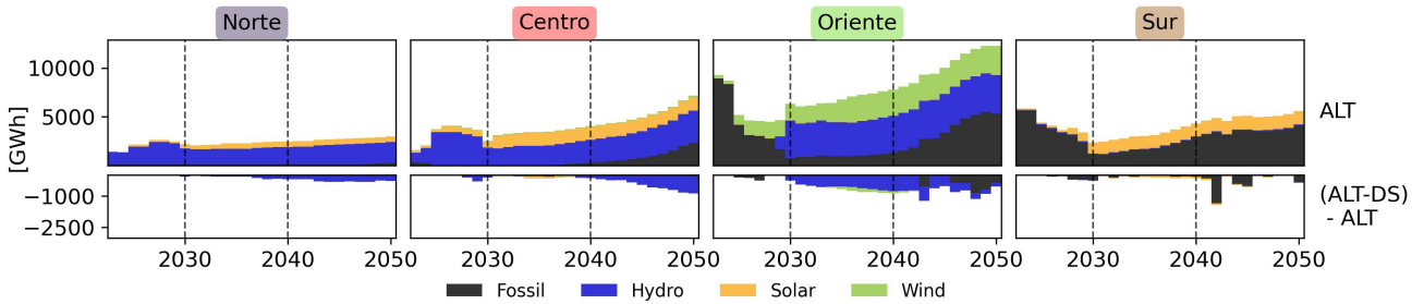
Figure 9: Evolution of regional projected annual electricity generation according to ALT scenario (upper row), and differences for ALT-DS scenario (lower row)
