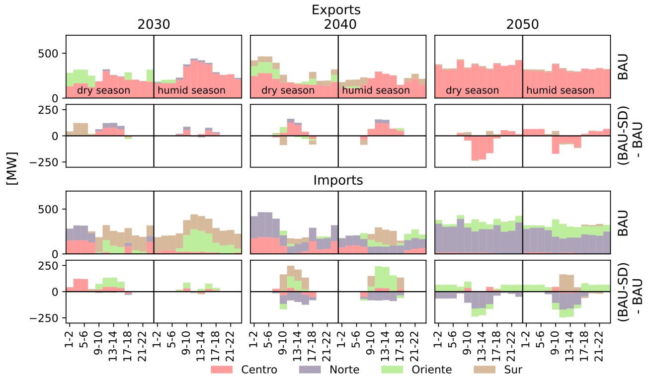
Figure 5: Daily profiles of inter regional exports and imports of power flow por BAU scenario (first and third row), and differences for BAU-SD scenario (second and fourth row)
