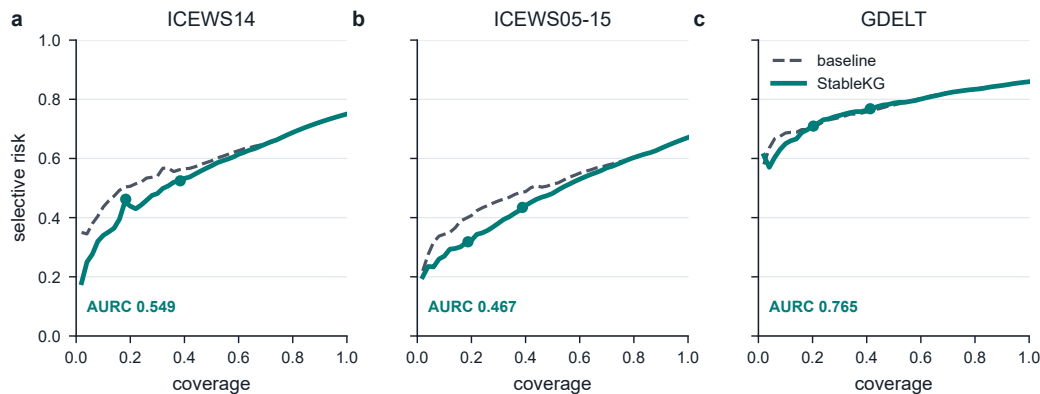
Figure 2: Selective risk-coverage curves. Each panel reports the test risk after sorting predictions by the belief-only baseline or the StableKG belief. Curves, points and AURC use calibration seed 0. Points show the actual test coverage and risk obtained at thresholds selected for 20% and 40% validation coverage; Tables S1 and S2 report seed aggregates and uncertainty.
