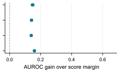
b TeRDy / ICEWS05-15
