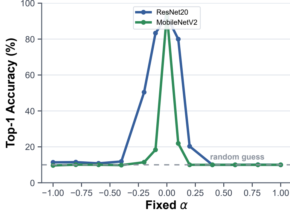
(b) CIFAR-10 Accuracy
