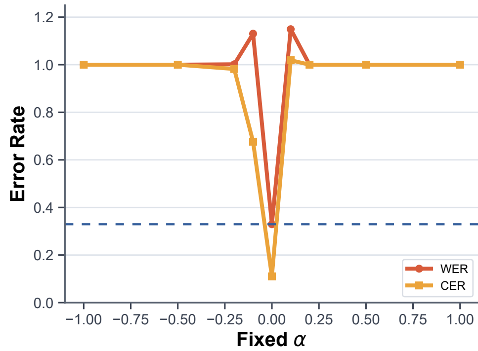
(c) VoxForge Whisper
