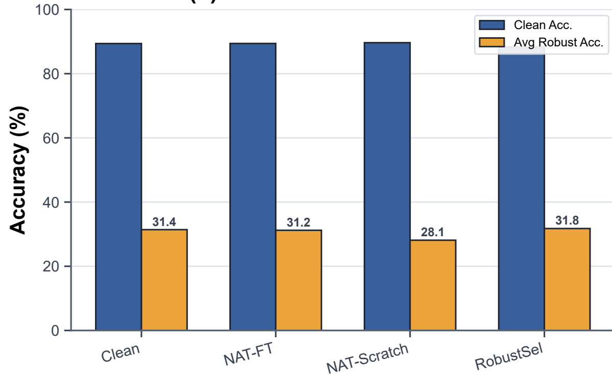
(a) CIFAR-10 NAT Baseline
