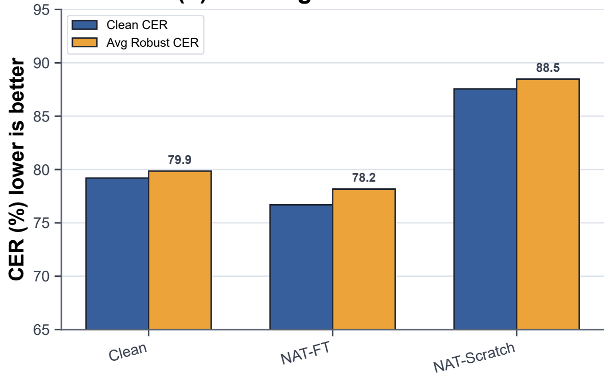
(b) VoxForge NAT Baseline
