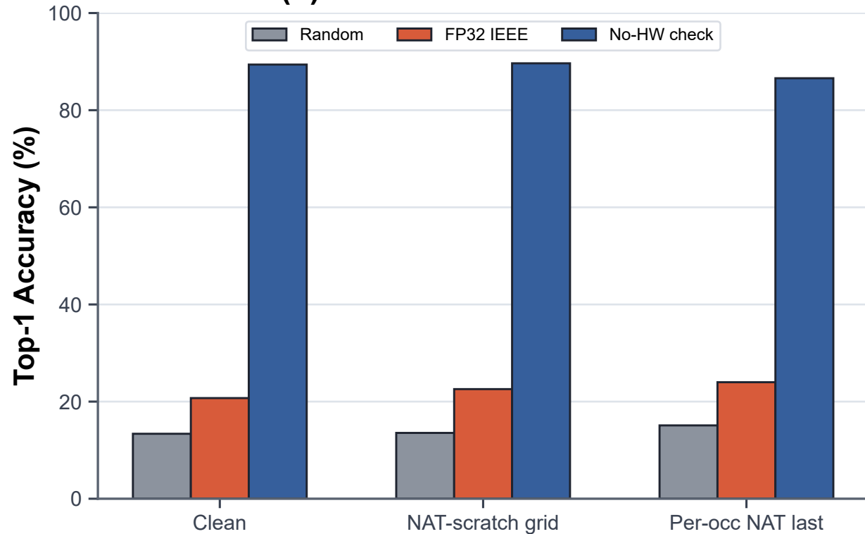
(a) FP32 Value-Plane Test
