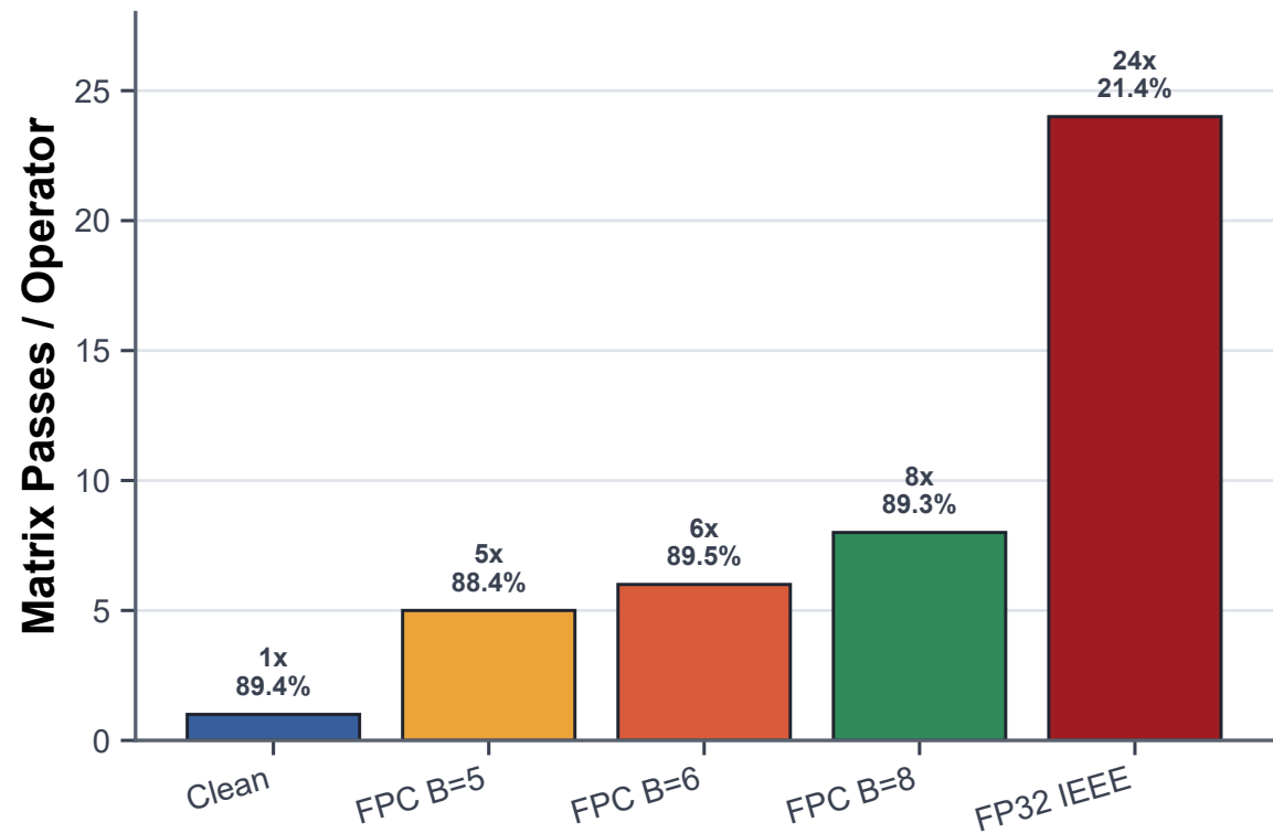
(b) Serial Compute Cost
