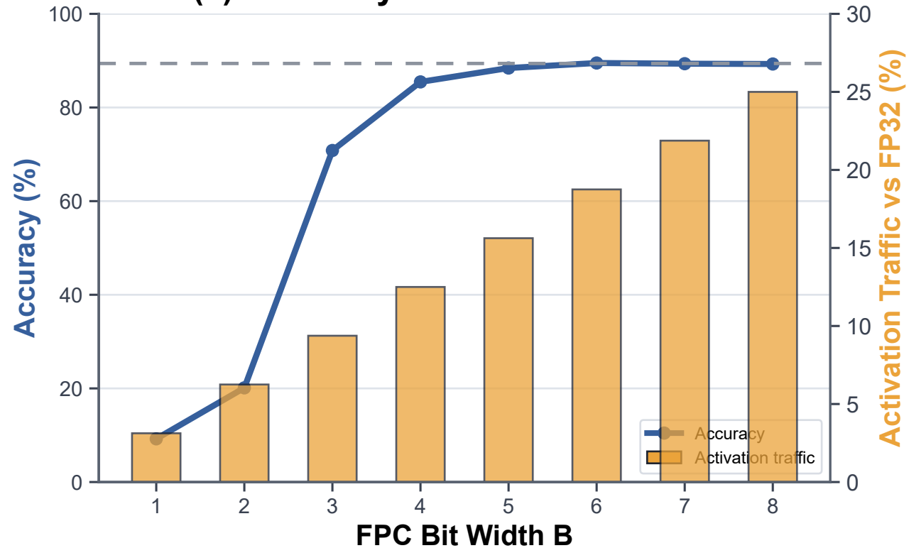
(a) Accuracy-Bandwidth Trade-off
