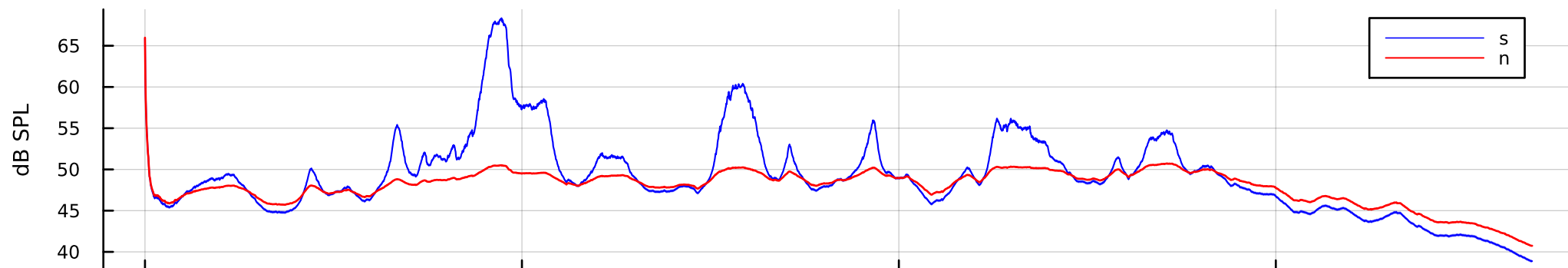
p257_003, bus noise, 7.5 dB SNR, band 13 (fc \approx 3619 Hz)
