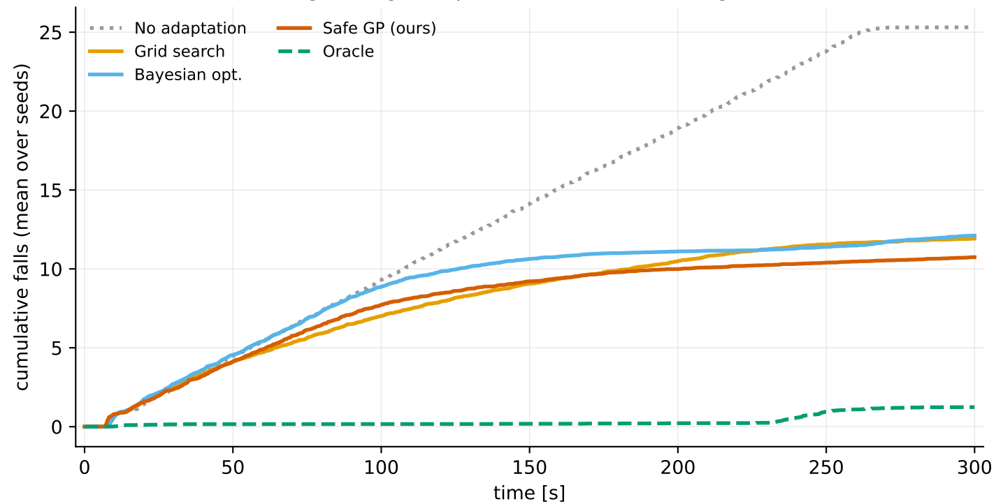
Continual leg-damage adaptation: falls accumulating over the bout
