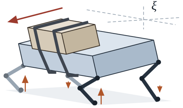
Fig. 1. Schematic of quadruped robot with base state \xi being perturbed by leg motion. Events such as payload shifts alter which parameters are optimal. Arrows at feet indicate compensation by virtual attitude controller.
