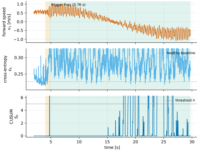
Fig. 5. Top : forward speed, which the tolerant gait carries slowly backward under the load. Middle : the attitude cross-entropy \epsilon_k rests at its baseline and rises when the shift tilts the trunk (shaded orange until the trigger fires, green once the proposed gait is active). It settles above baseline rather than returning to it. Bottom : the CUSUM S_k crosses its threshold h within 0.76 s, is held at zero through the settle window, and re-crosses later in the bout without drawing a second adaptation, the monitor having latched for the event.
