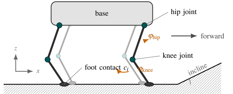
Fig. 1. The Laikago quadruped, its trunk base state \xi , and the twelve leg joints driven by the CPG.
