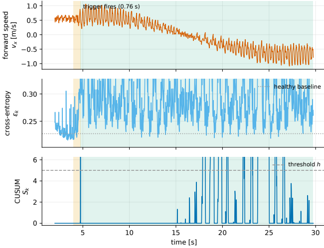
Fig. 5. Top: forward speed, which the tolerant gait carries slowly backward under the load. Middle: the attitude cross-entropy \epsilon_k rests at its baseline and rises when the shift tilts the trunk (shaded orange until the trigger fires, green once the proposed gait is active). It settles above baseline rather than returning to it. Bottom: the CUSUM S_k crosses its threshold h within 0.76 s, is held at zero through the settle window, and re-crosses later in the bout without drawing a second adaptation, the monitor having latched for the event.
