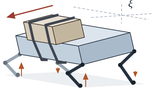
Fig. 1. Schematic of quadruped robot with base state \xi being perturbed by leg motion. Events such as payload shifts alter which parameters are optimal. Arrows at feet indicate compensation by virtual attitude controller.
