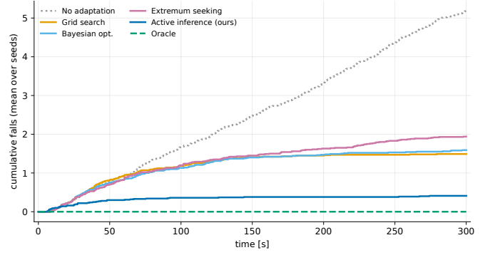
Fig. 3. Cumulative falls over a 300s continual bout under the persistent payload shift (mean over one hundred seeds). Holding the incumbent gait accrues falls throughout. The three arms that must trial a candidate on the loaded robot (grid search, Bayesian optimization, extremum seeking) find a tolerant gait early but pay for the search first. Our agent, which screens each candidate against a memory of past falls before committing to it, falls far less.
