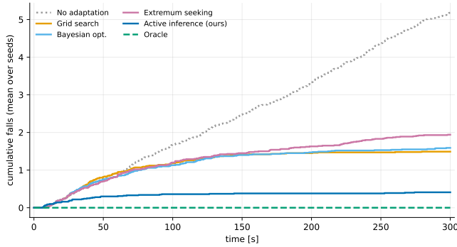
Fig. 3. Cumulative falls over a 300 s continual bout under the persistent payload shift (mean over one hundred seeds). Holding the incumbent gait accrues falls throughout. The three arms that must trial a candidate on the loaded robot (grid search, Bayesian optimization, extremum seeking) find a tolerant gait early but pay for the search first. Our agent, which screens each candidate against a memory of past falls before committing to it, falls far less.
