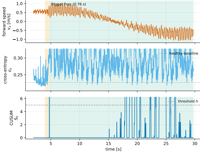
Fig. 5. The uprightness-only trigger over one payload shift (ours). Top : forward speed, which the tolerant gait carries slowly backward under the load. Middle : the attitude cross-entropy \epsilon_k rests at its healthy baseline and rises when the shift tilts the trunk (shaded orange until the trigger fires, green once the proposed gait is active); it settles above baseline rather than returning to it. Bottom : the CUSUM S_k crosses its threshold h within 0.76 s, is held at zero through the settle window, and re-crosses later in the bout without drawing a second adaptation, the monitor having latched for the event.
