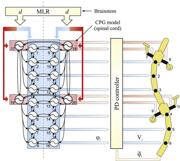
Fig. 1. Salamander CPG model tested with a amphibious salamander-like robot (Ijspeert et al., 2007). The model is composed of 20 amplitude-controlled phase oscillators. The oscillators receive a drive d signal representing the descending stimulation from the Mesencephalic Locomotor Region (MLR) in the brain stem. The outputs of the CPG are desired joint angle positions \phi_i that are used by a Proportional-Derivative (PD) feedback controller ( V_i are the voltages applied to the motors and \tilde{\phi}_i are the actual joint angles measured from incremental encoders). For details see the text and (Ijspeert et al., 2007).
