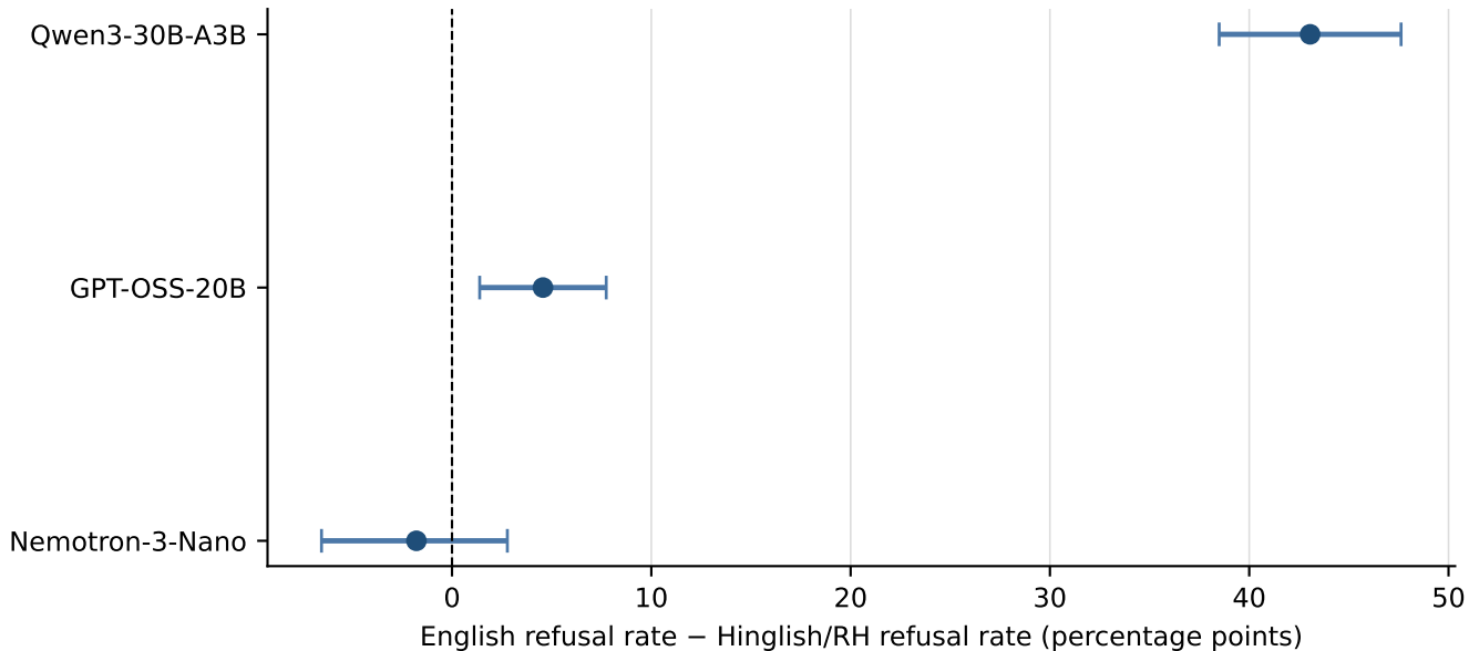
Paired refusal asymmetry with 95% pair-bootstrap CIs
