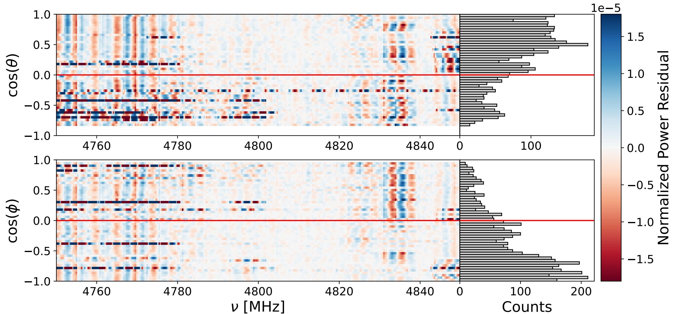
Bank 0 ann: 4750-4850 MHz
