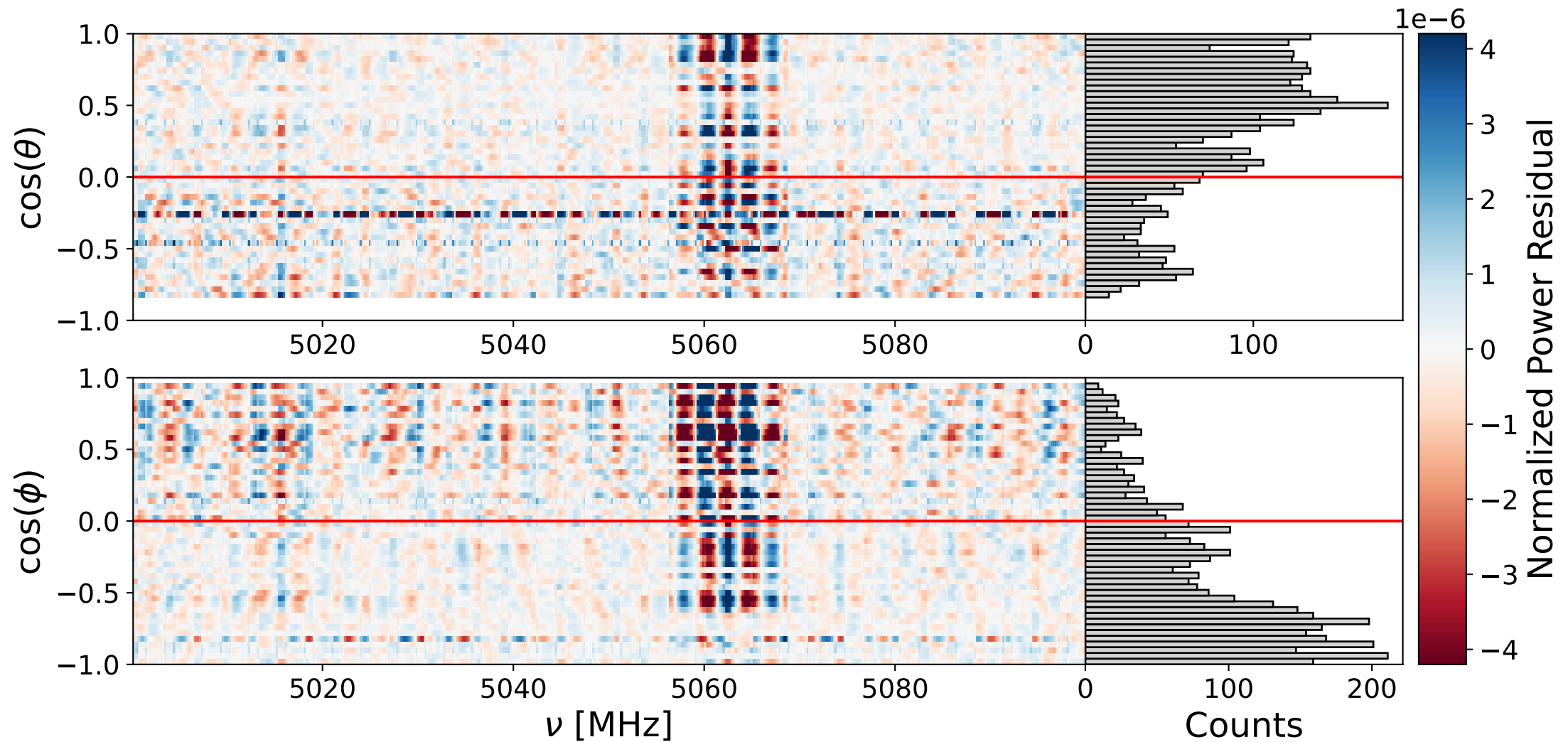
Bank 1 ann: 5000-5100 MHz
