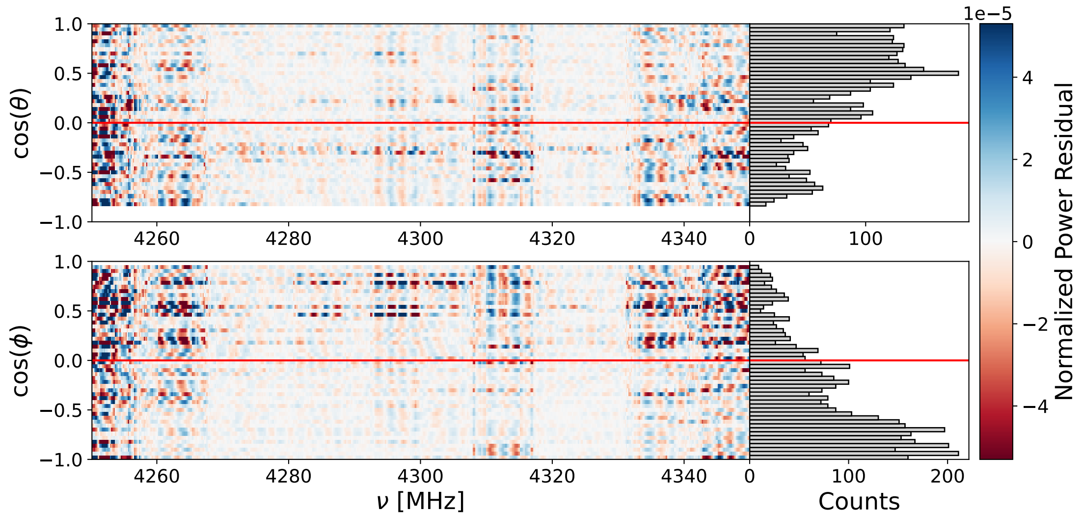
Bank 0 ann: 4250-4350 MHz
