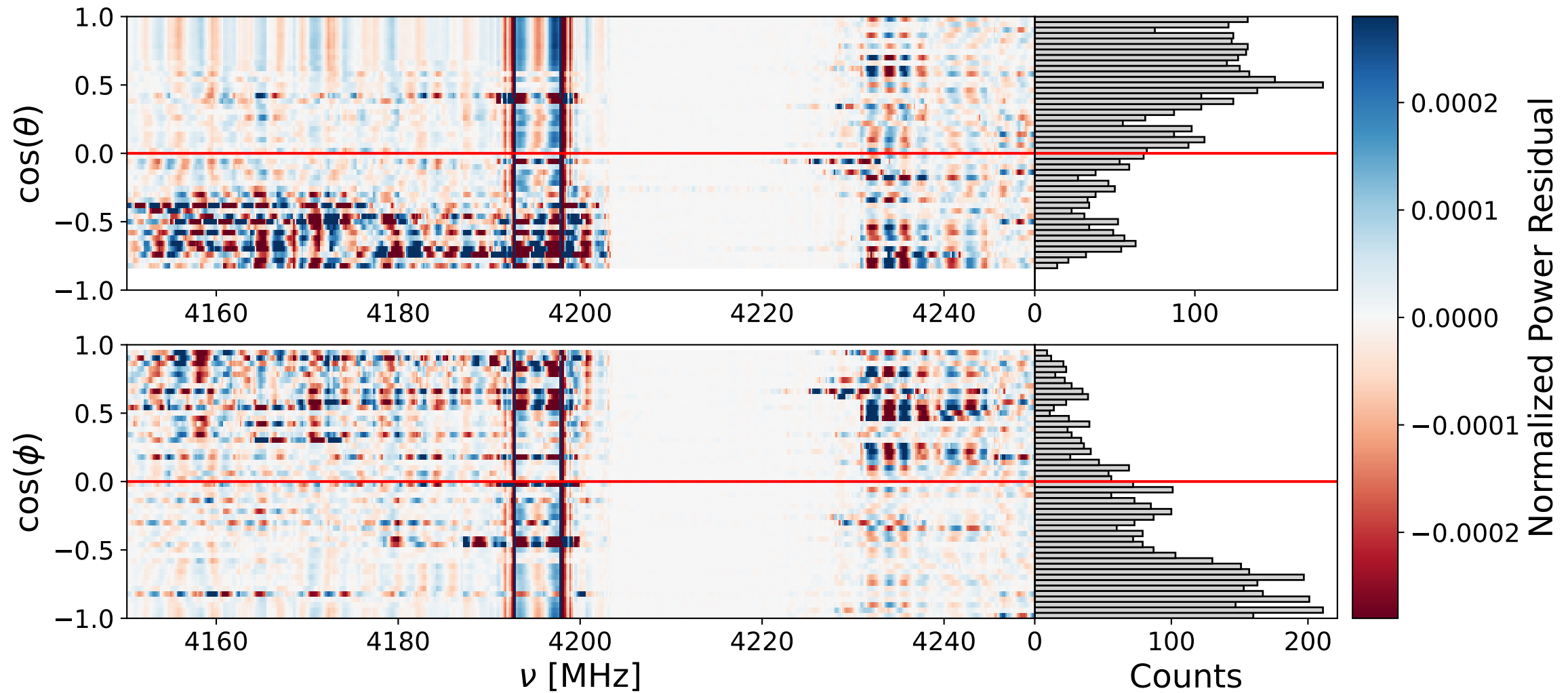
Bank 0 ann: 4150-4250 MHz
