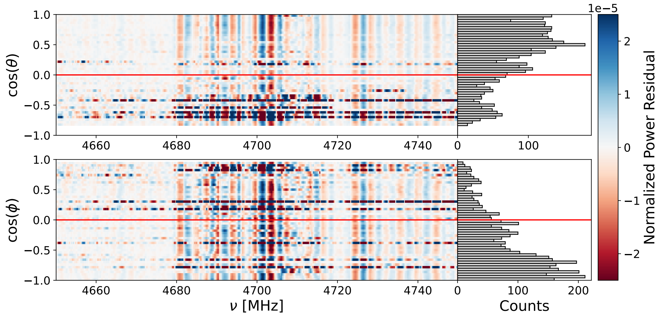
Bank 0 ann: 4650-4750 MHz
