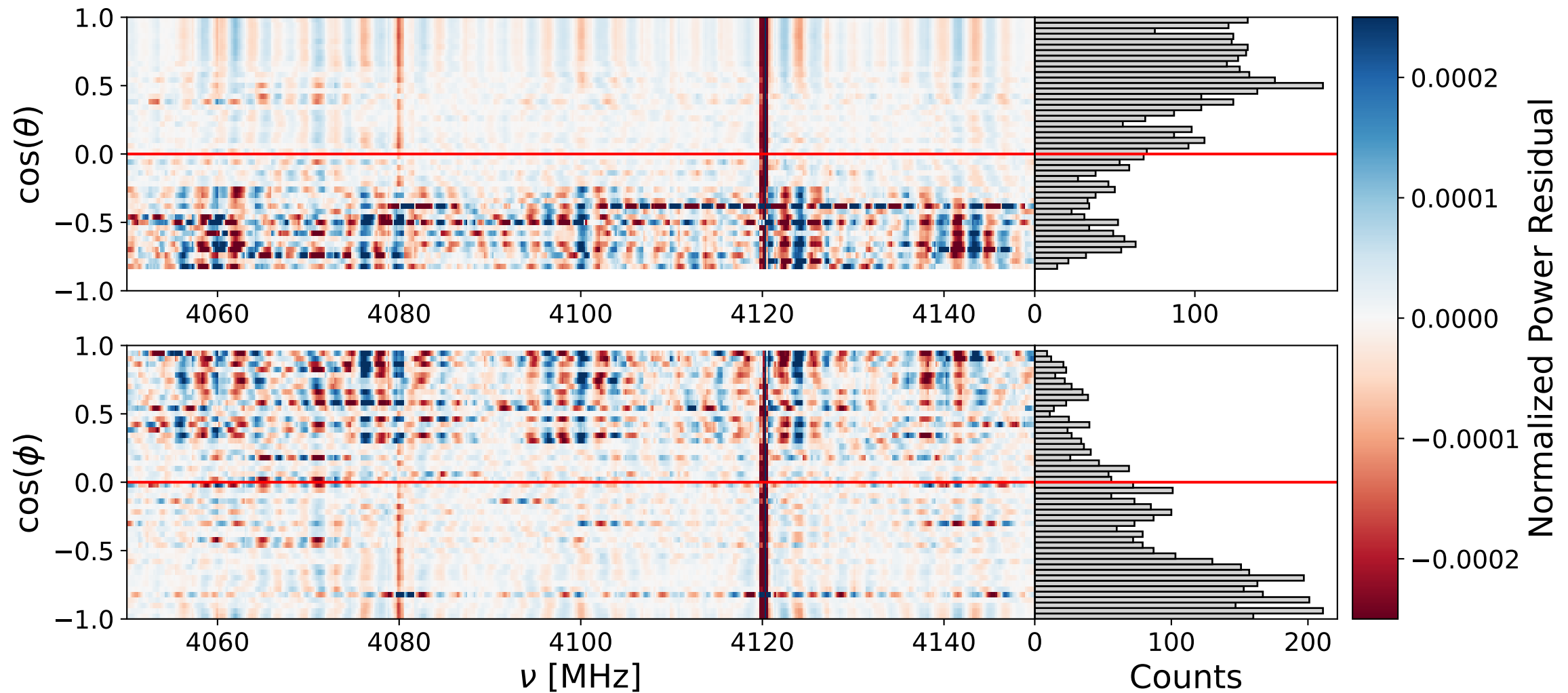
Bank 0 ann: 4050-4150 MHz
