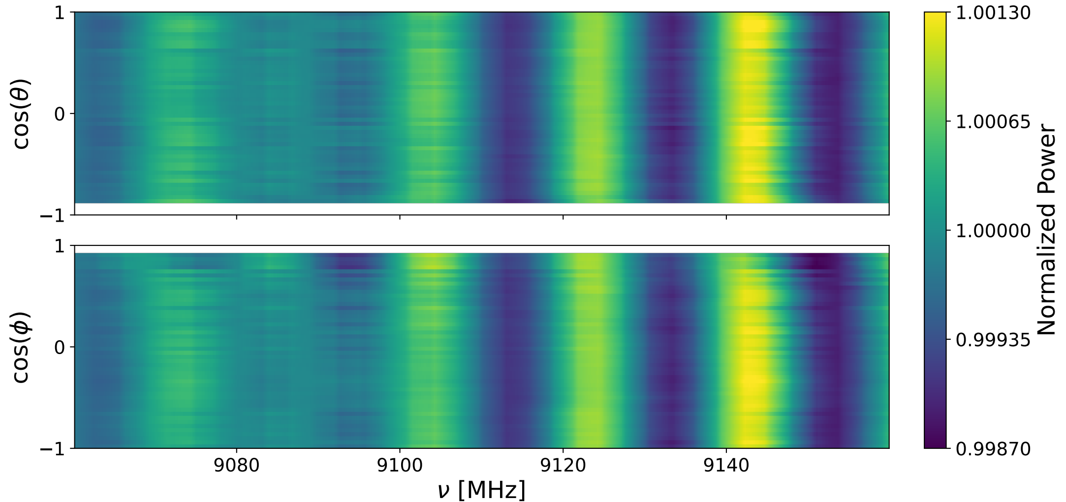
Bank 1 decay: 9060-9160 MHz
