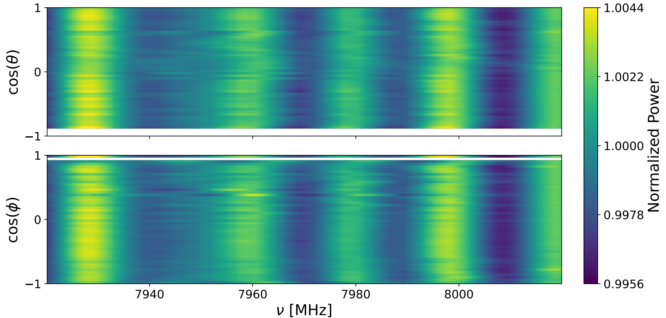
Bank 0 decay: 7920-8020 MHz
