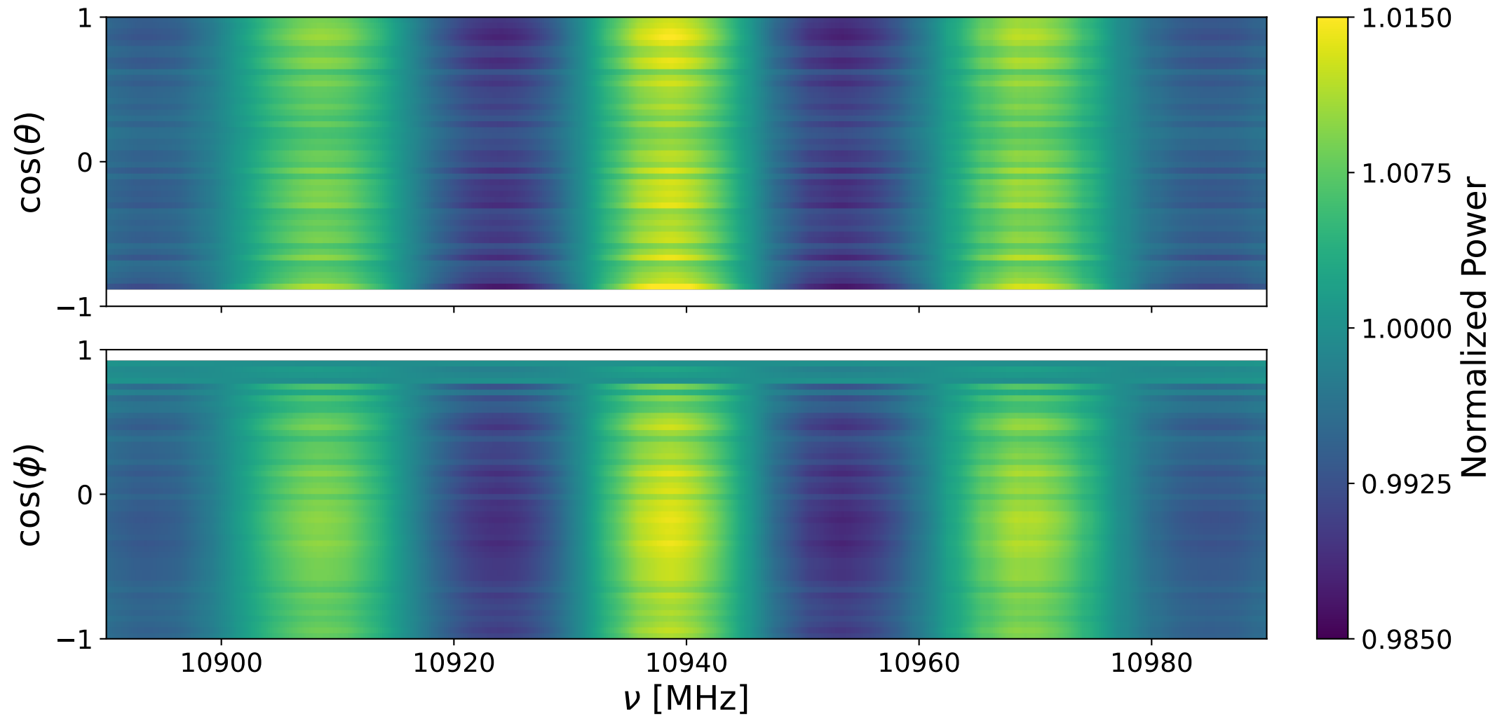
Bank 2 decay: 10890-10990 MHz
