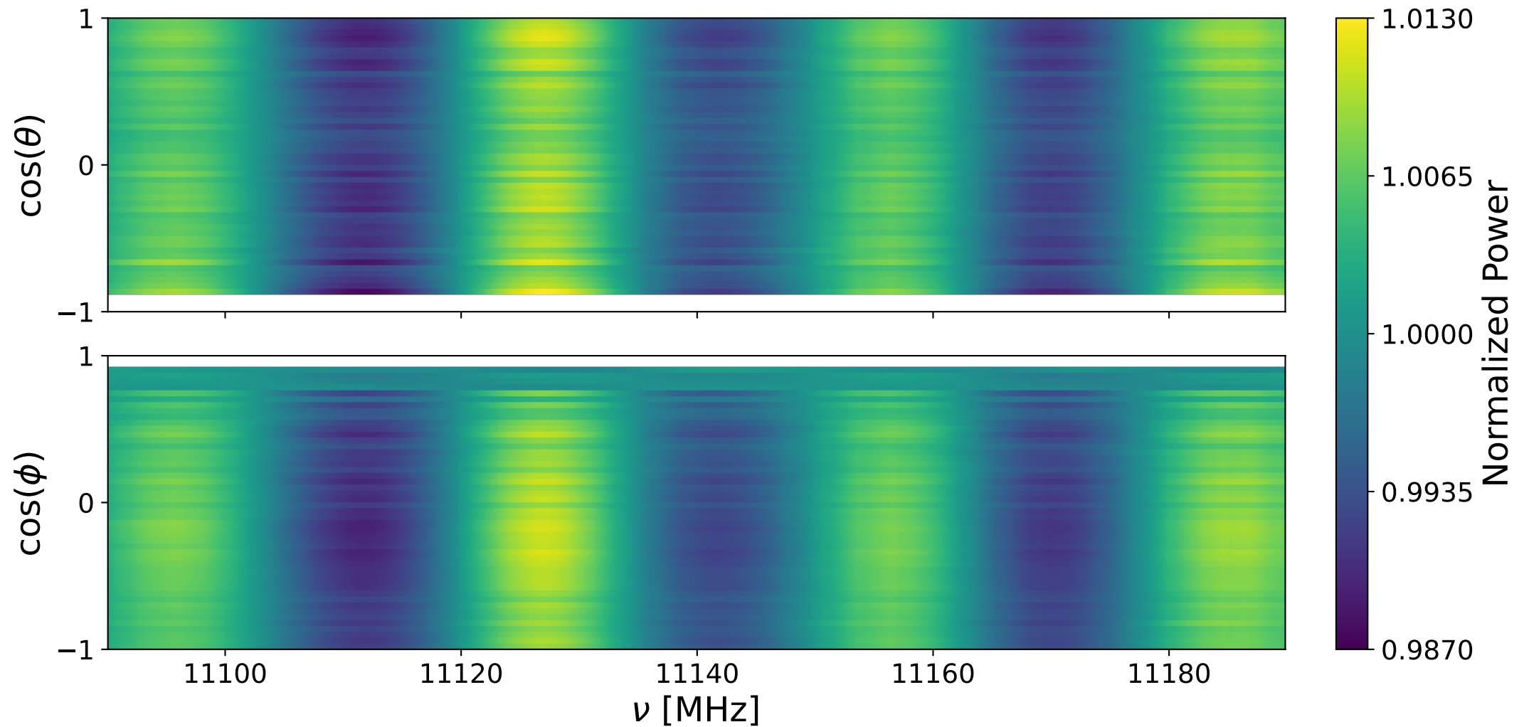
Bank 2 decay: 11090-11190 MHz
