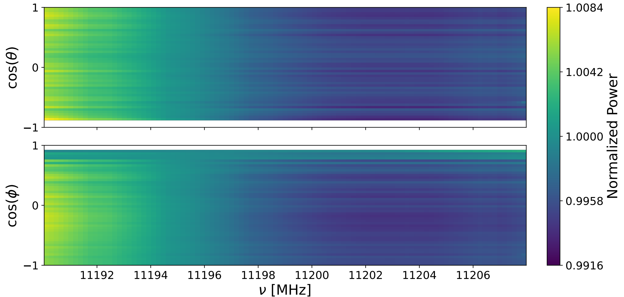
Bank 2 decay: 11190-11208 MHz
