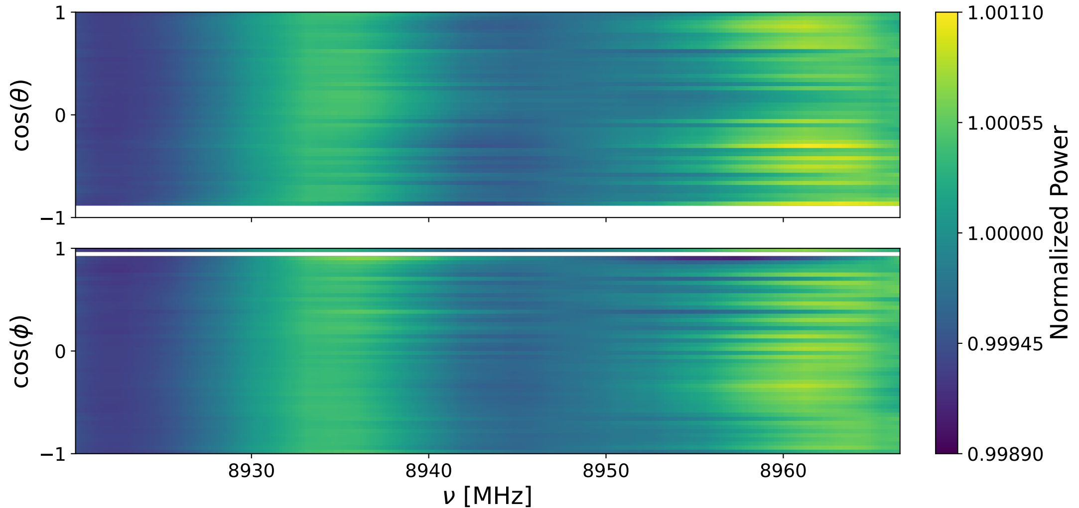
Bank 0 decay: 8920-8967 MHz
