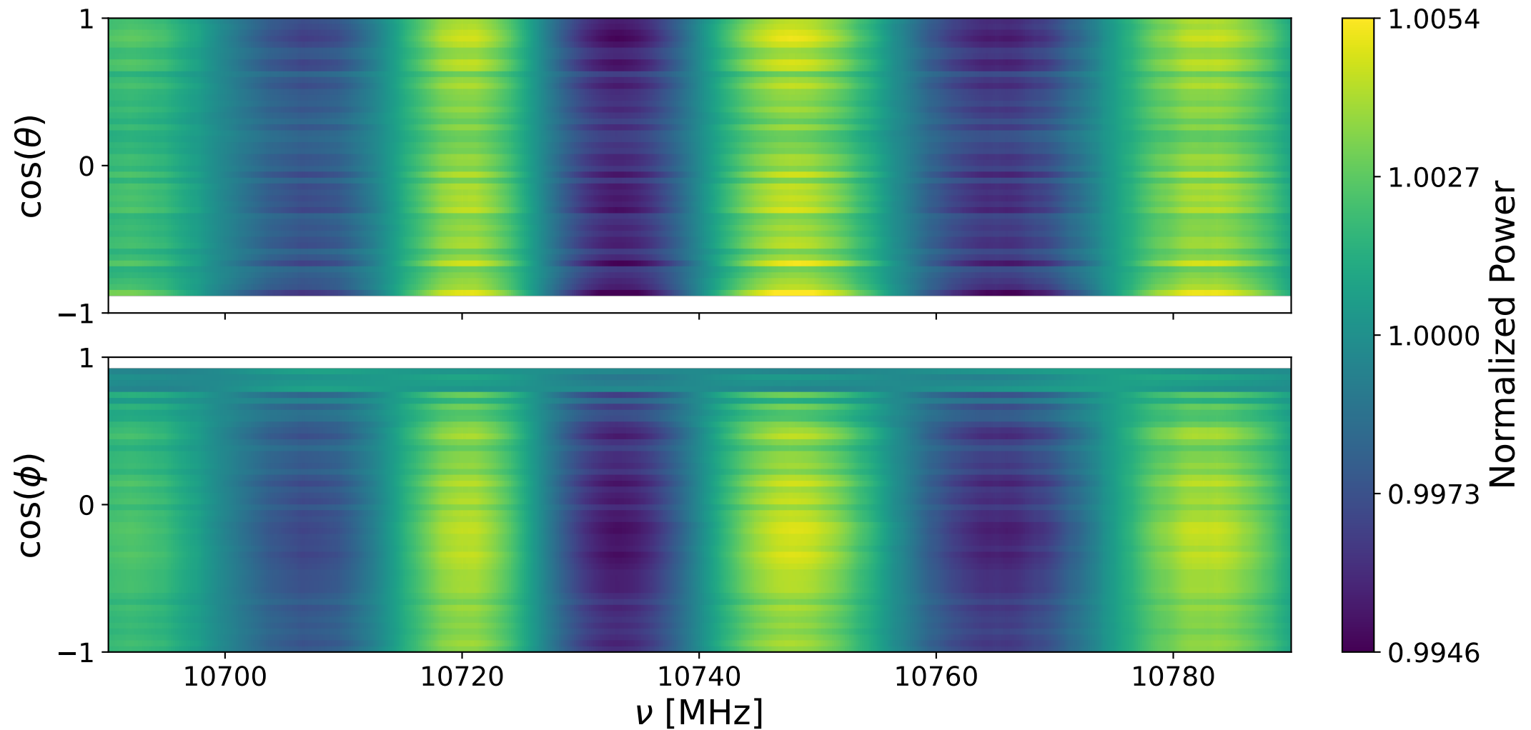
Bank 2 decay: 10690-10790 MHz
