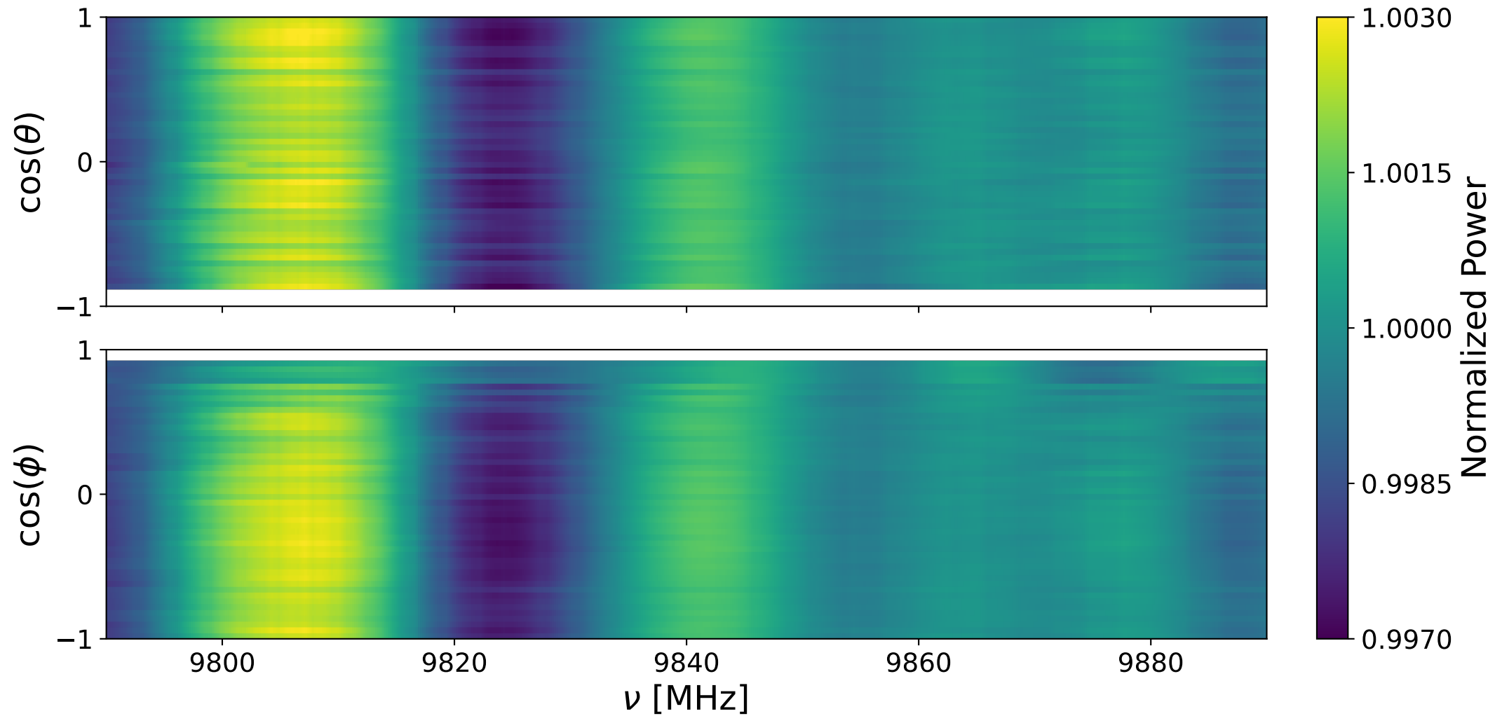
Bank 2 decay: 9790-9890 MHz
