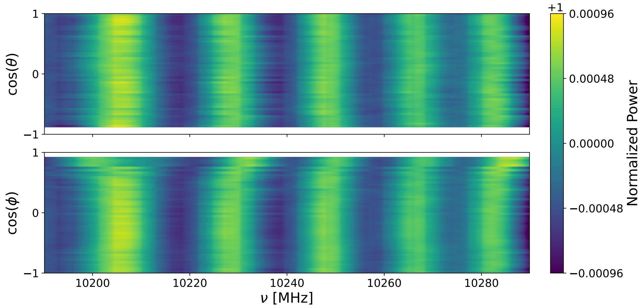
Bank 2 decay: 10190-10290 MHz
