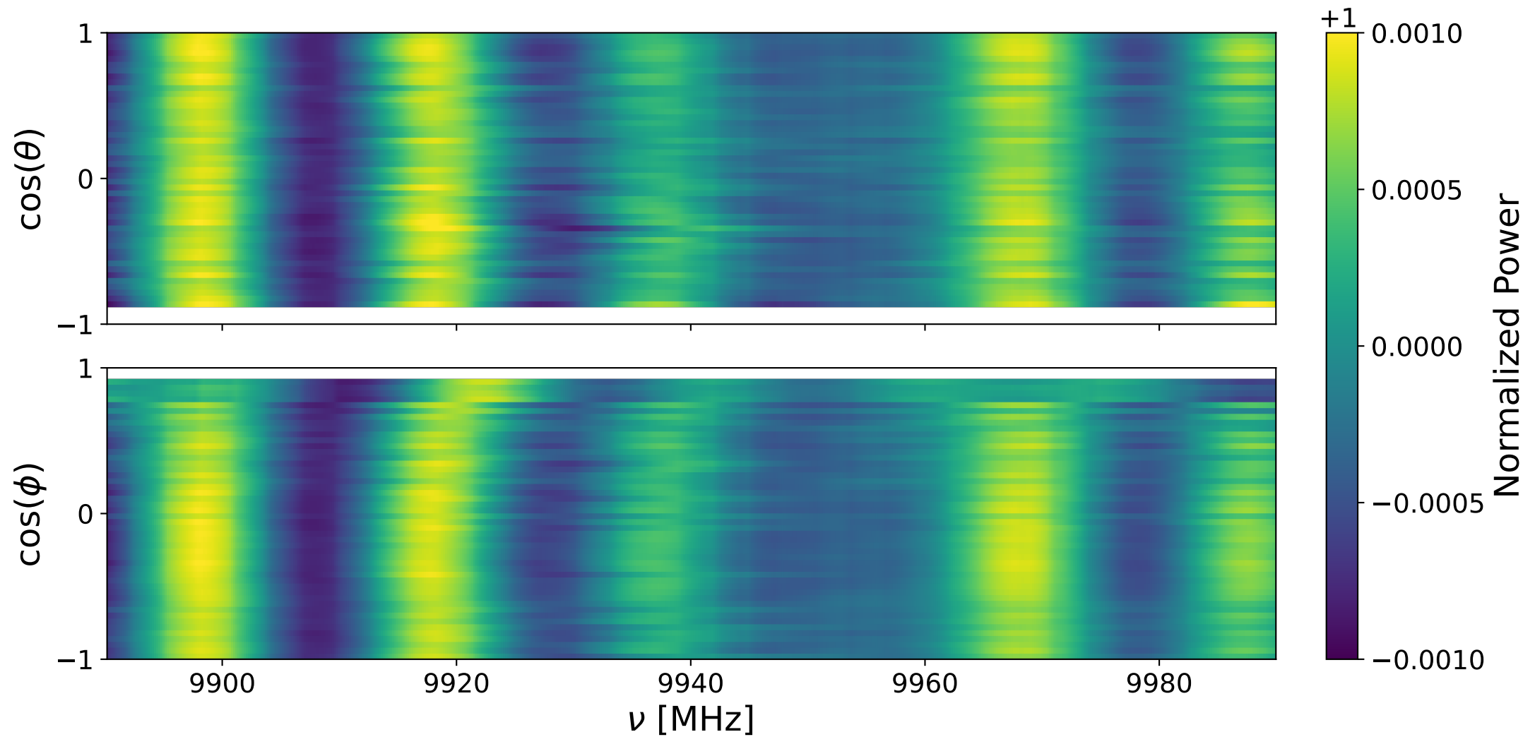
Bank 2 decay: 9890-9990 MHz
