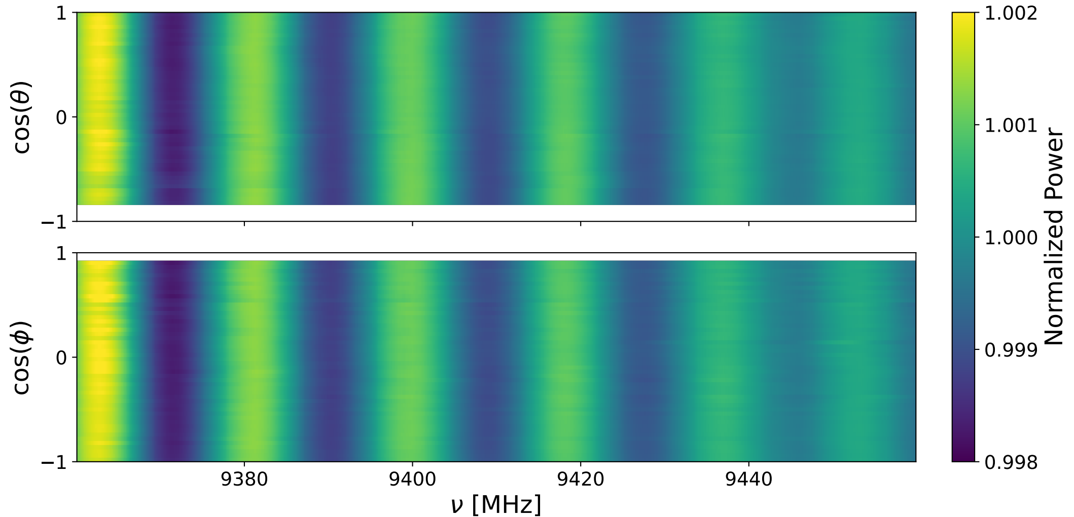
Bank 1 ann: 9360-9460 MHz
