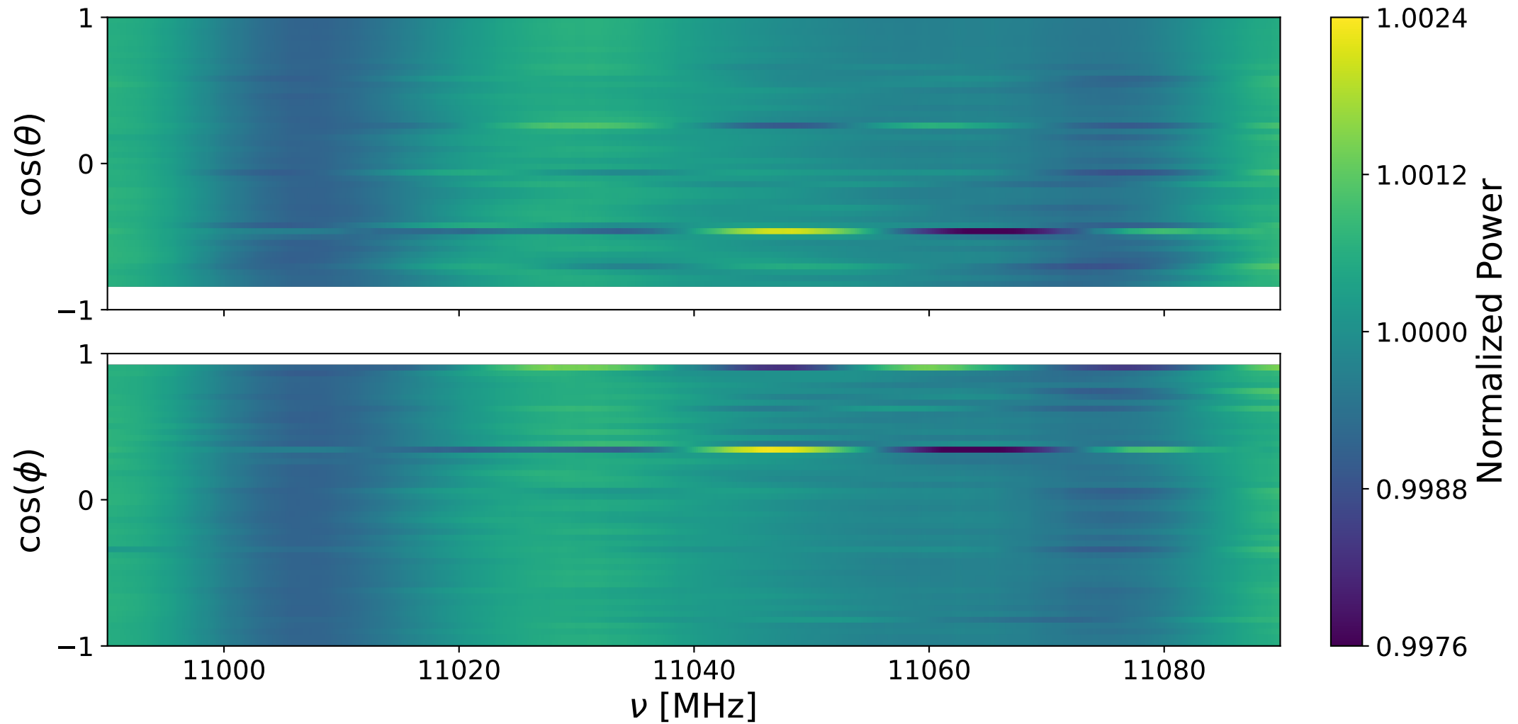
Bank 2 decay: 10990-11090 MHz
