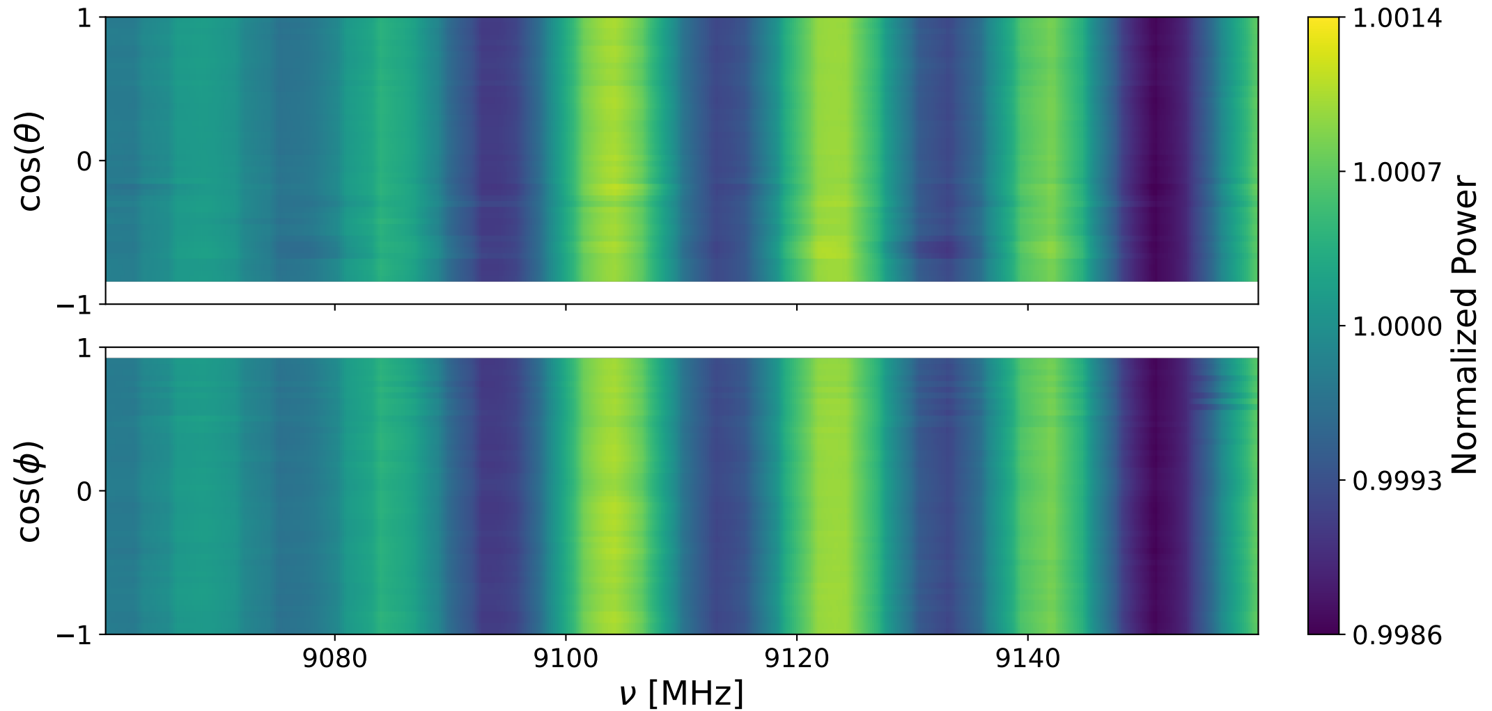
Bank 1 decay: 9060-9160 MHz
