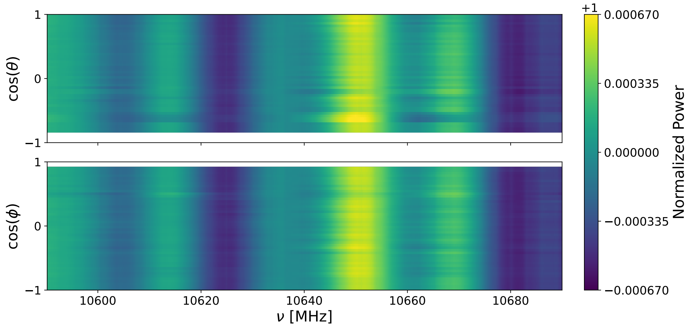
Bank 2 decay: 10590-10690 MHz
