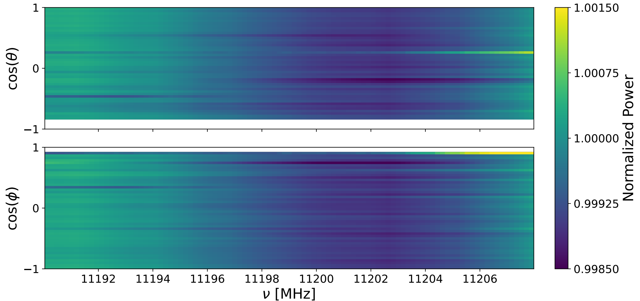
Bank 2 decay: 11190-11208 MHz
