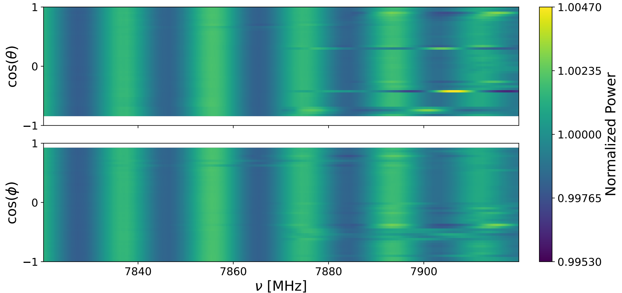
Bank 0 decay: 7820-7920 MHz
