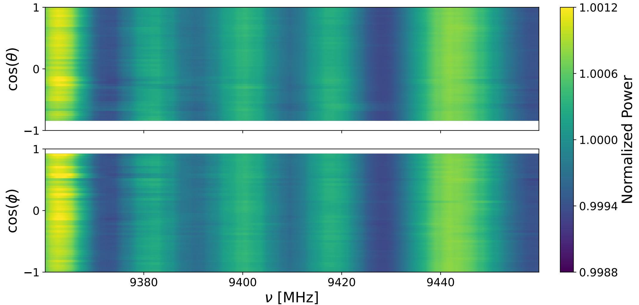
Bank 1 decay: 9360-9460 MHz
