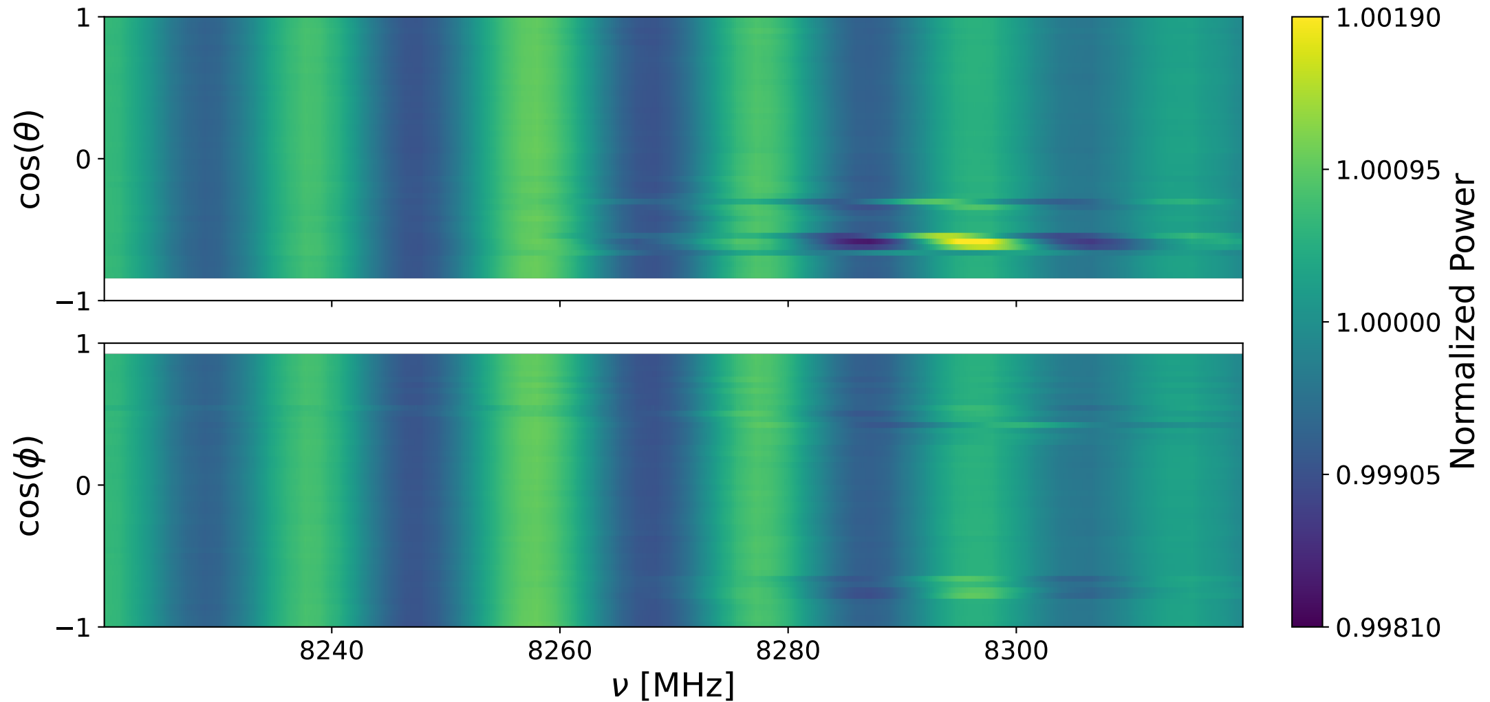
Bank 0 decay: 8220-8320 MHz
