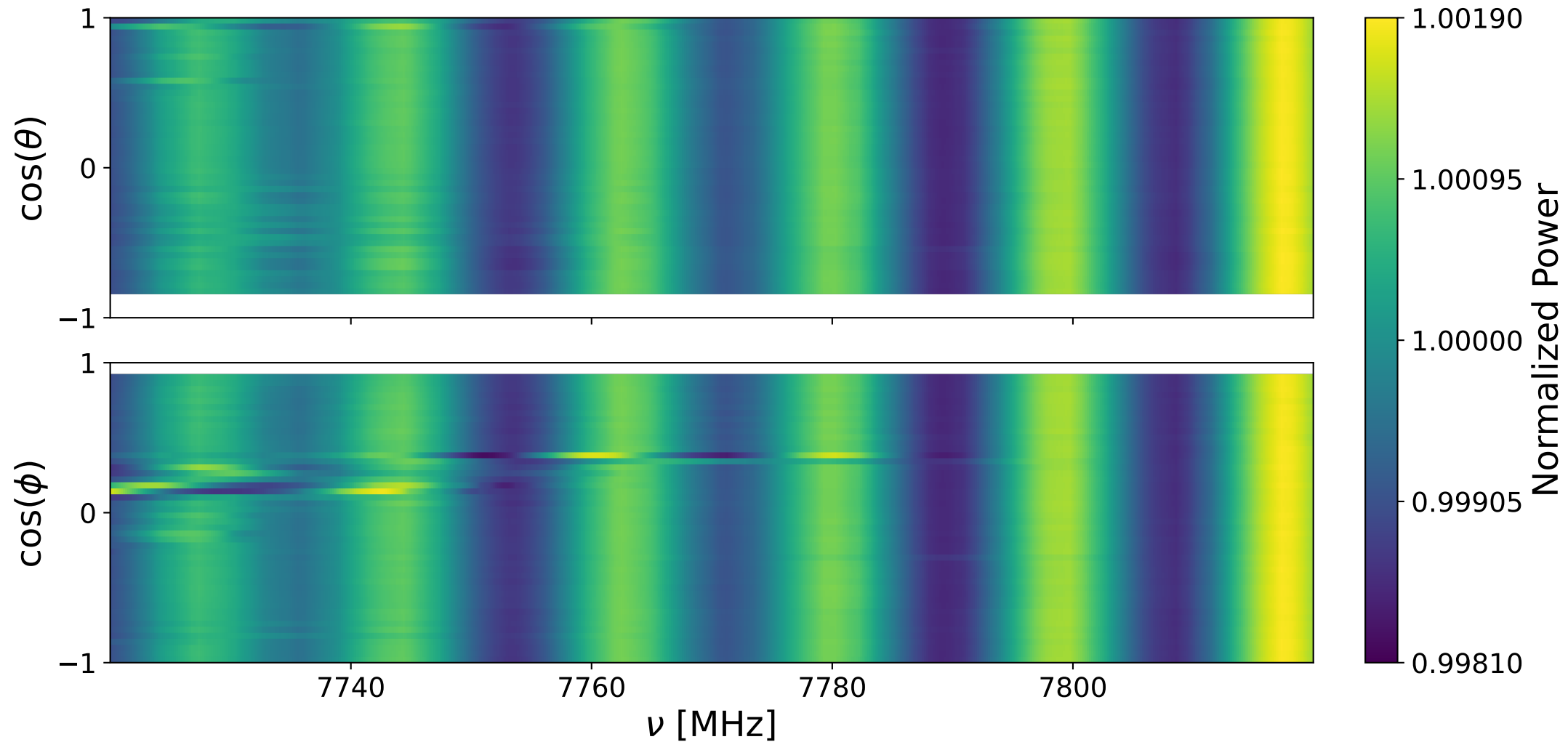
Bank 0 decay: 7720-7820 MHz
