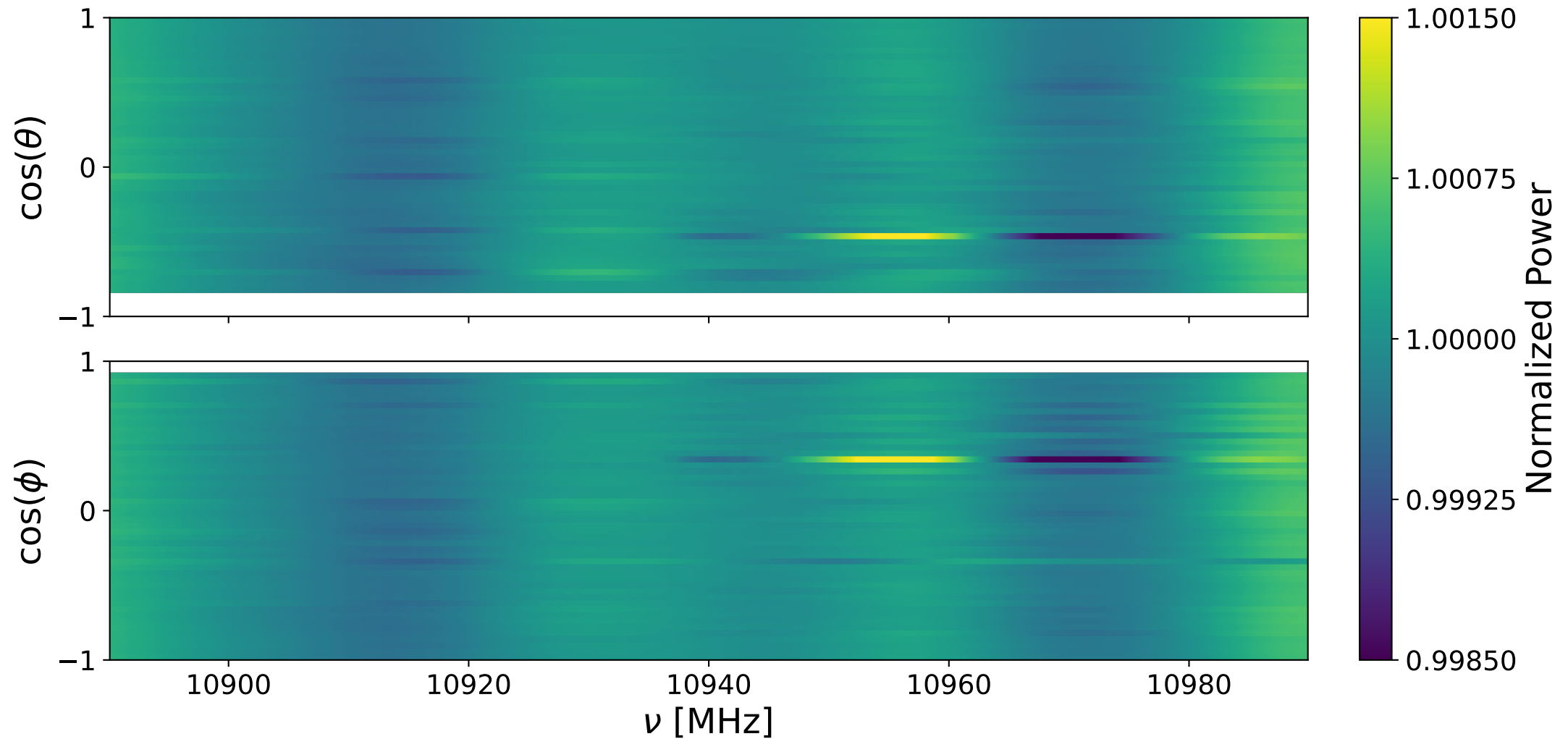
Bank 2 decay: 10890-10990 MHz
