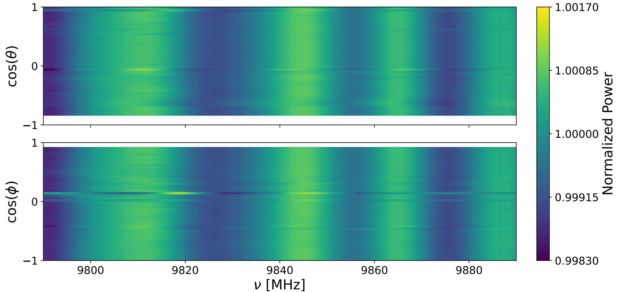
Bank 2 decay: 9790-9890 MHz
