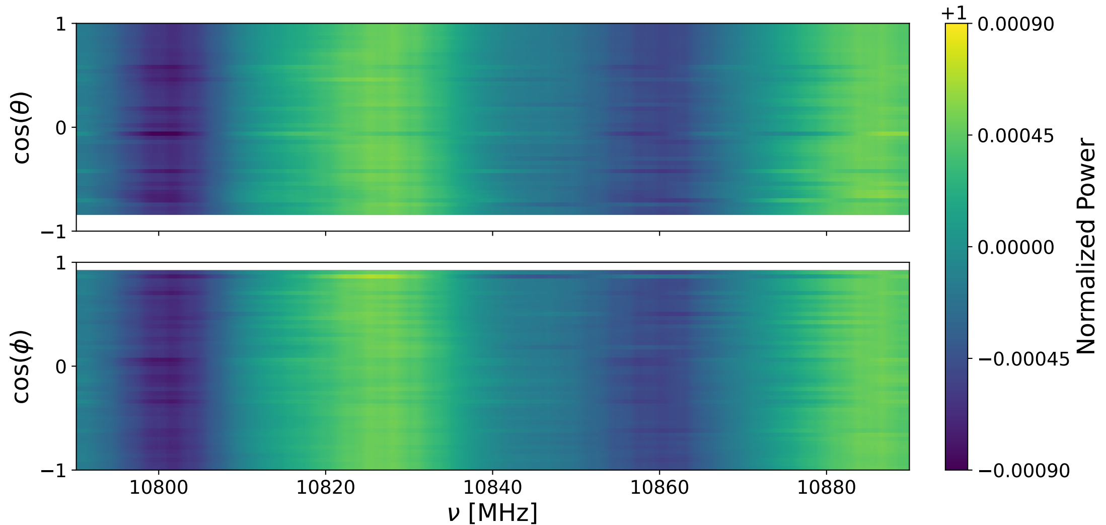
Bank 2 decay: 10790-10890 MHz
