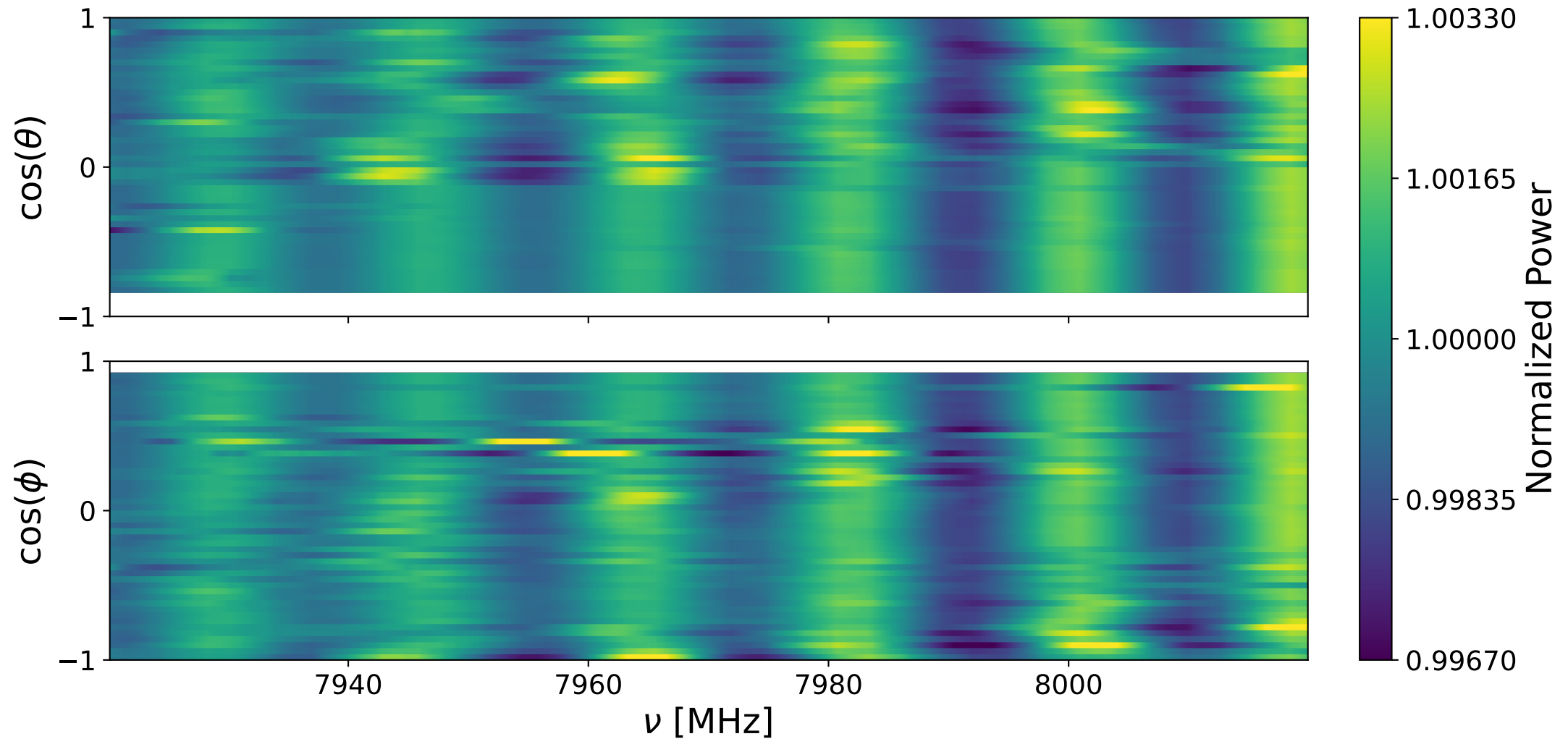
Bank 0 decay: 7920-8020 MHz
