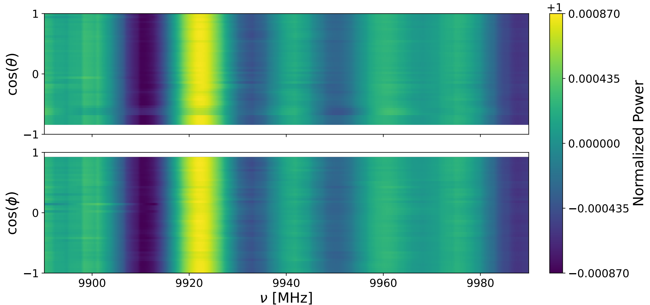
Bank 2 decay: 9890-9990 MHz
