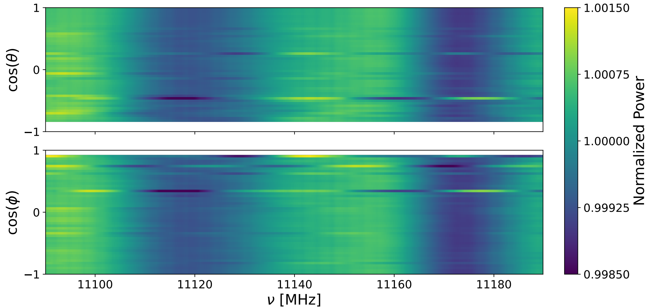
Bank 2 decay: 11090-11190 MHz
