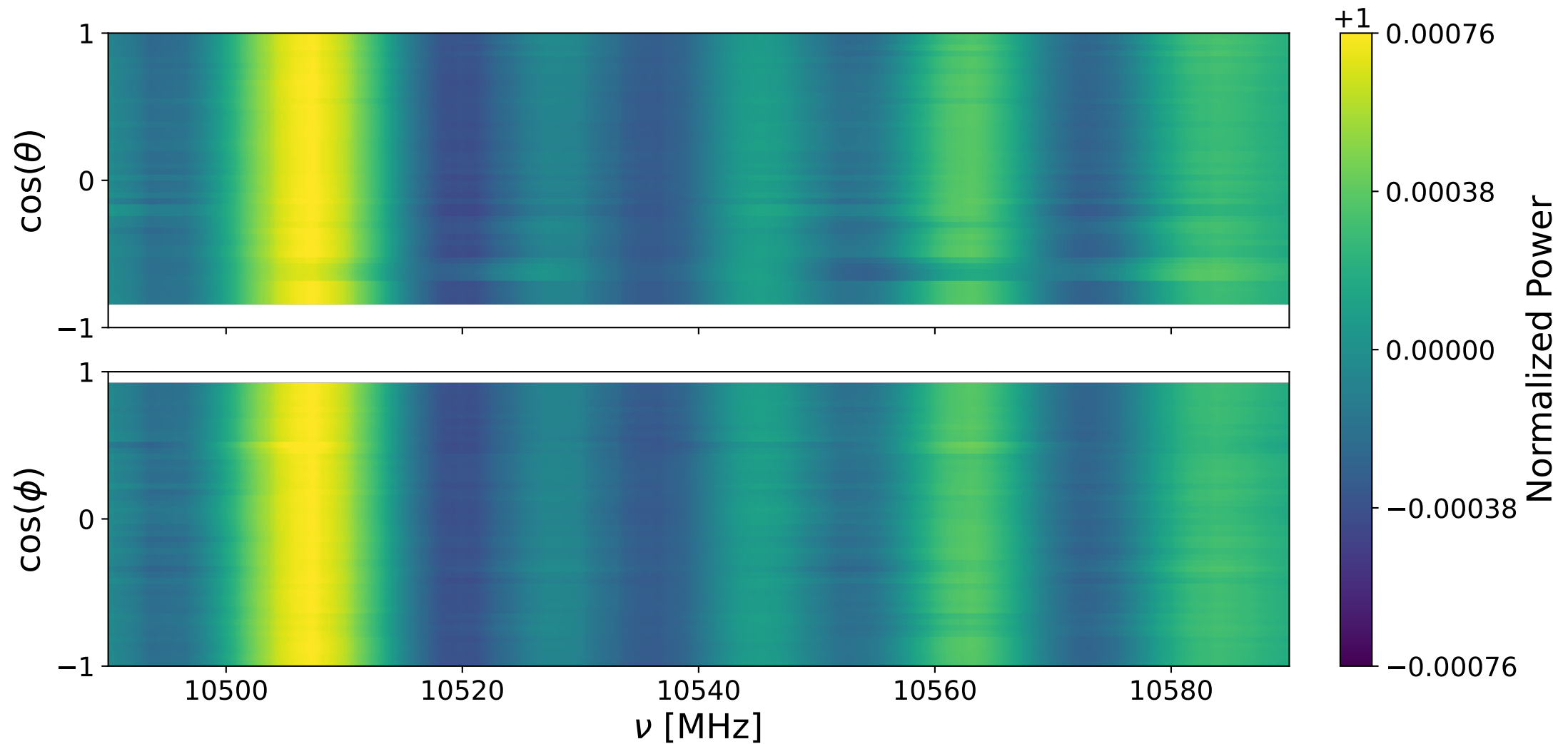
Bank 2 decay: 10490-10590 MHz
