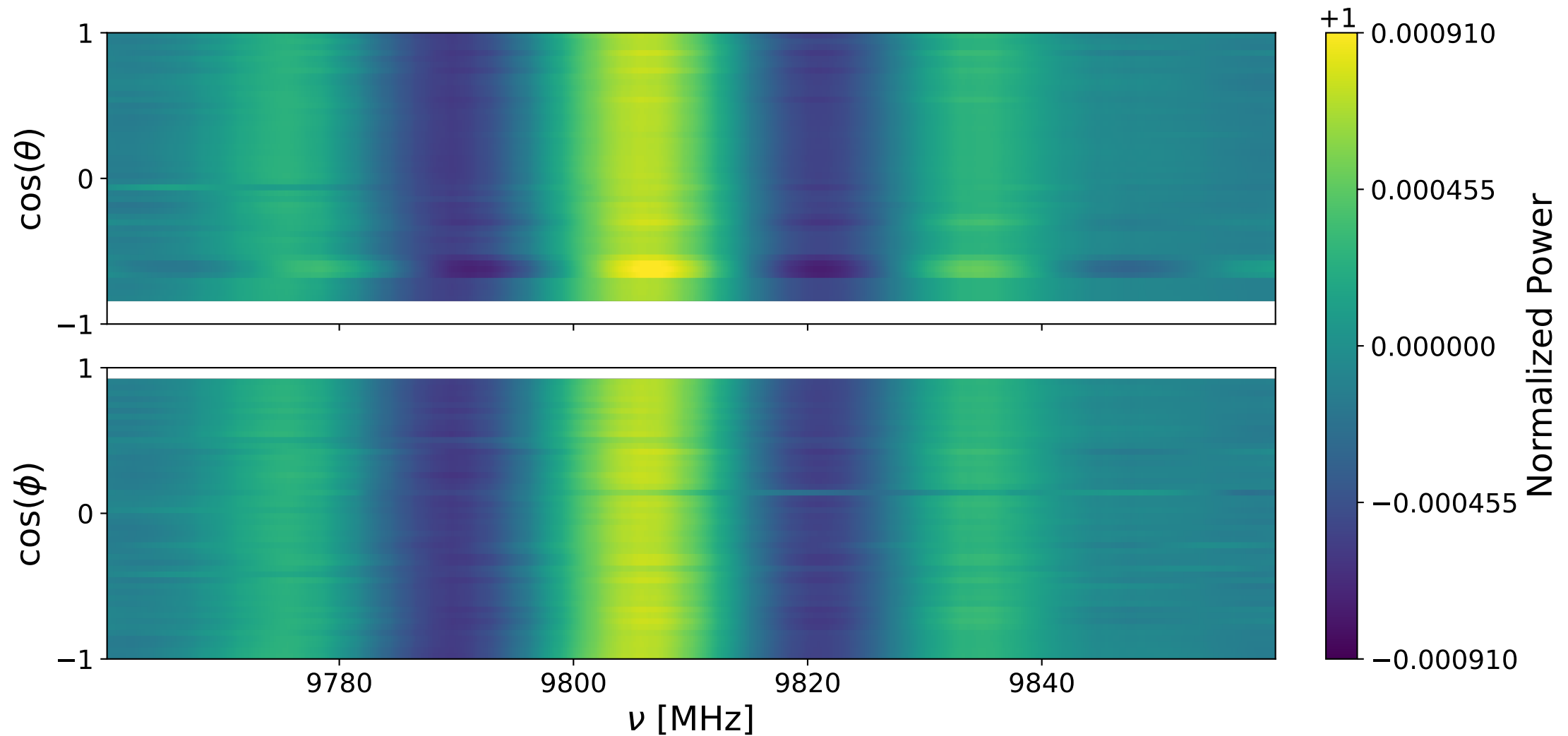
Bank 1 decay: 9760-9860 MHz
