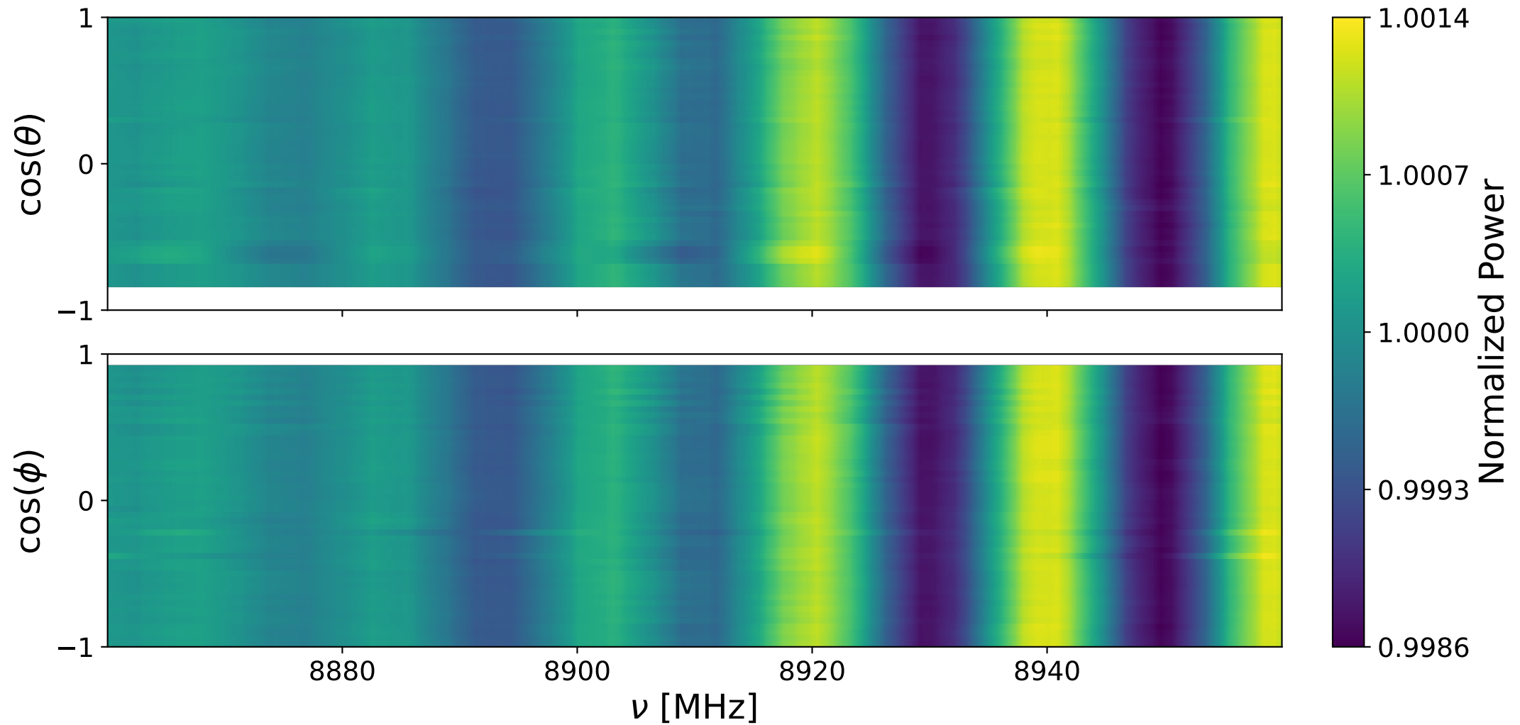
Bank 1 decay: 8860-8960 MHz
