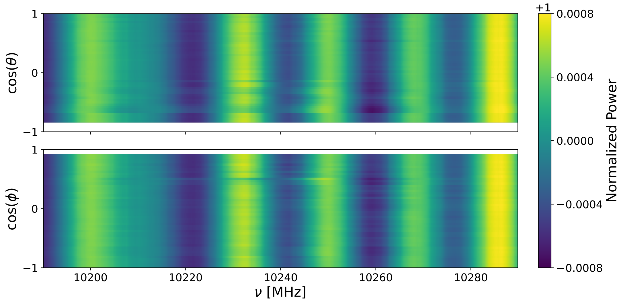
Bank 2 decay: 10190-10290 MHz
