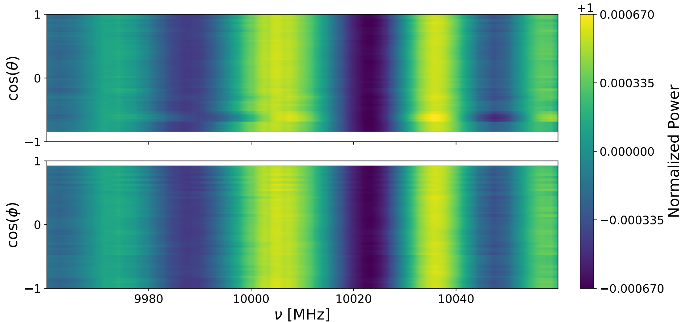
Bank 1 decay: 9960-10060 MHz
