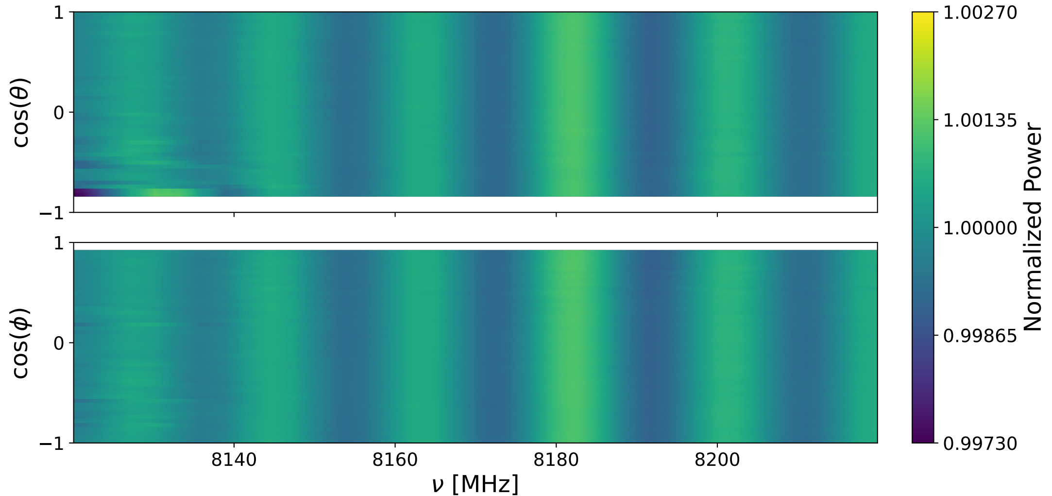
Bank 0 decay: 8120-8220 MHz
