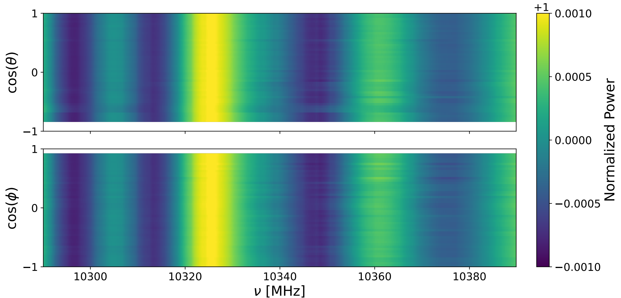
Bank 2 decay: 10290-10390 MHz
