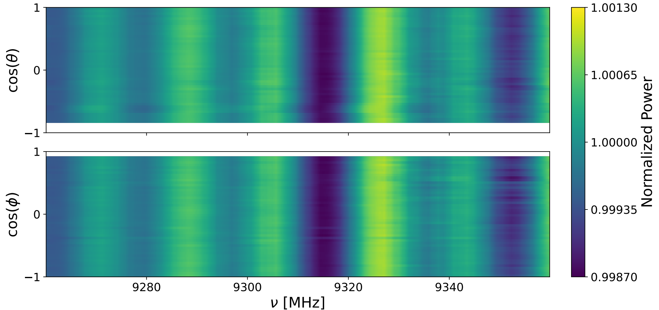
Bank 1 decay: 9260-9360 MHz
