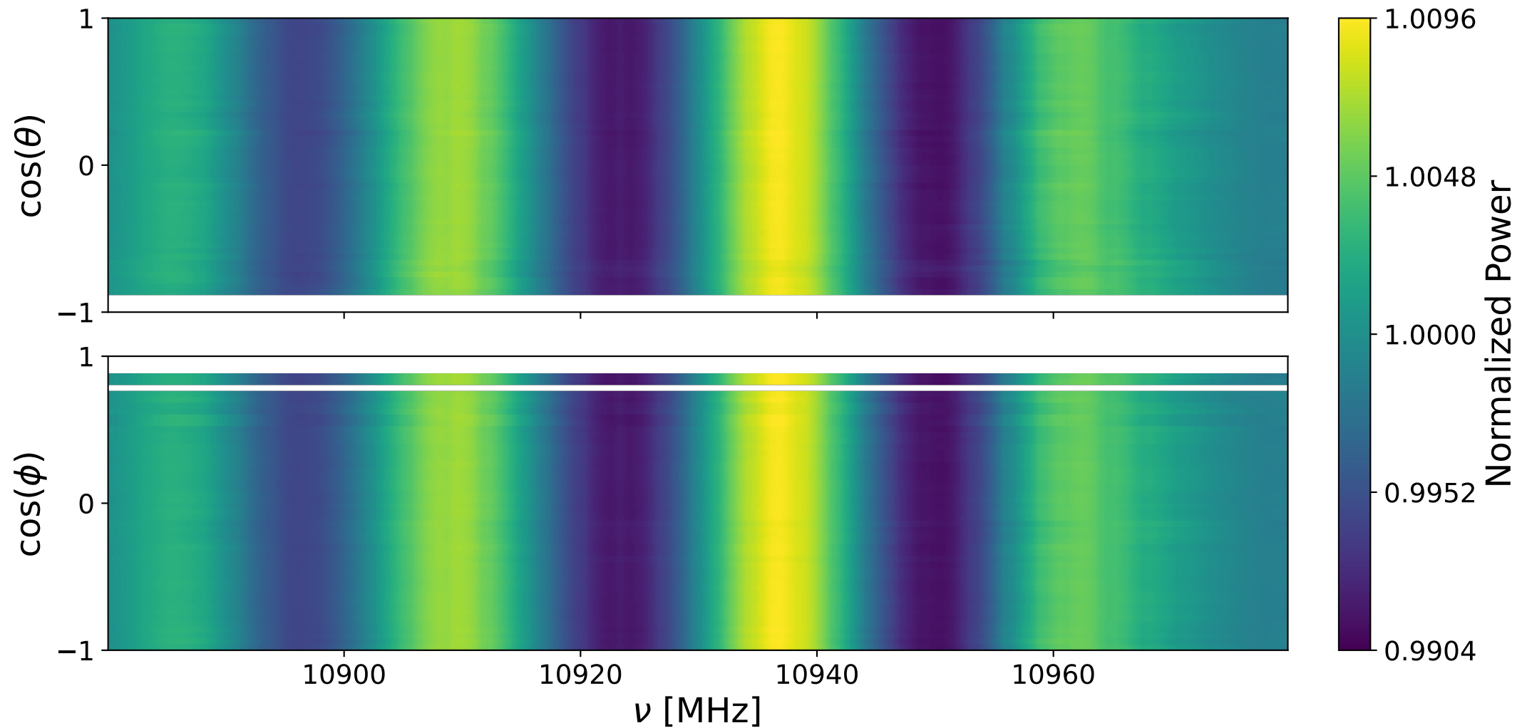
Bank 2 ann: 10880-10980 MHz
