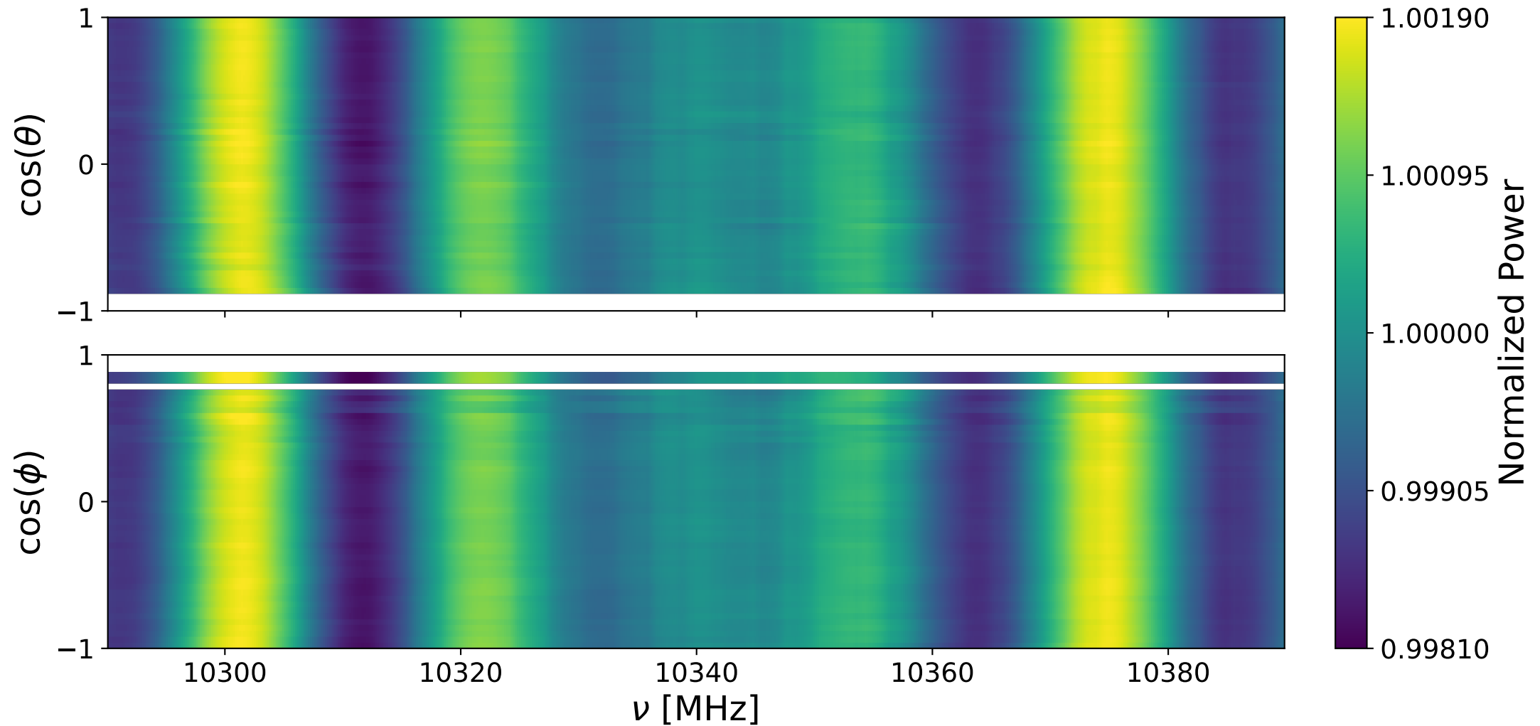
Bank 2 decay: 10290-10390 MHz
