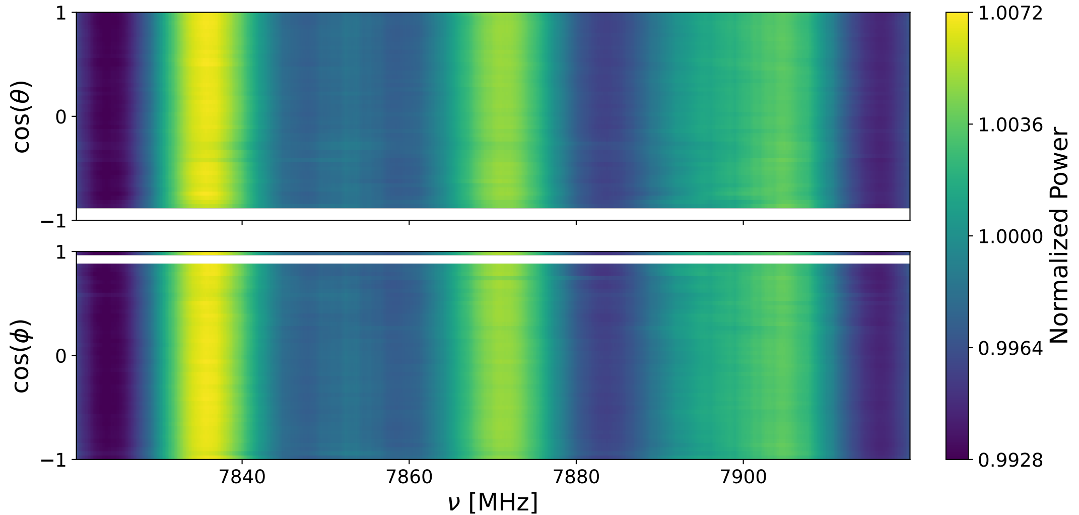
Bank 0 decay: 7820-7920 MHz
