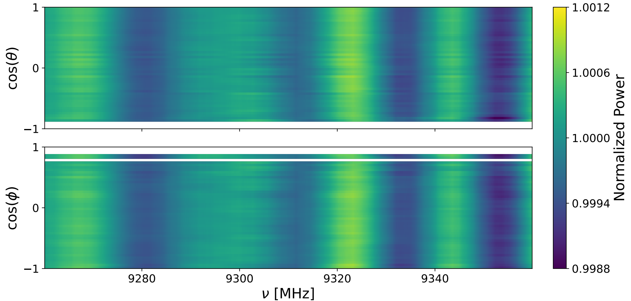
Bank 1 decay: 9260-9360 MHz
